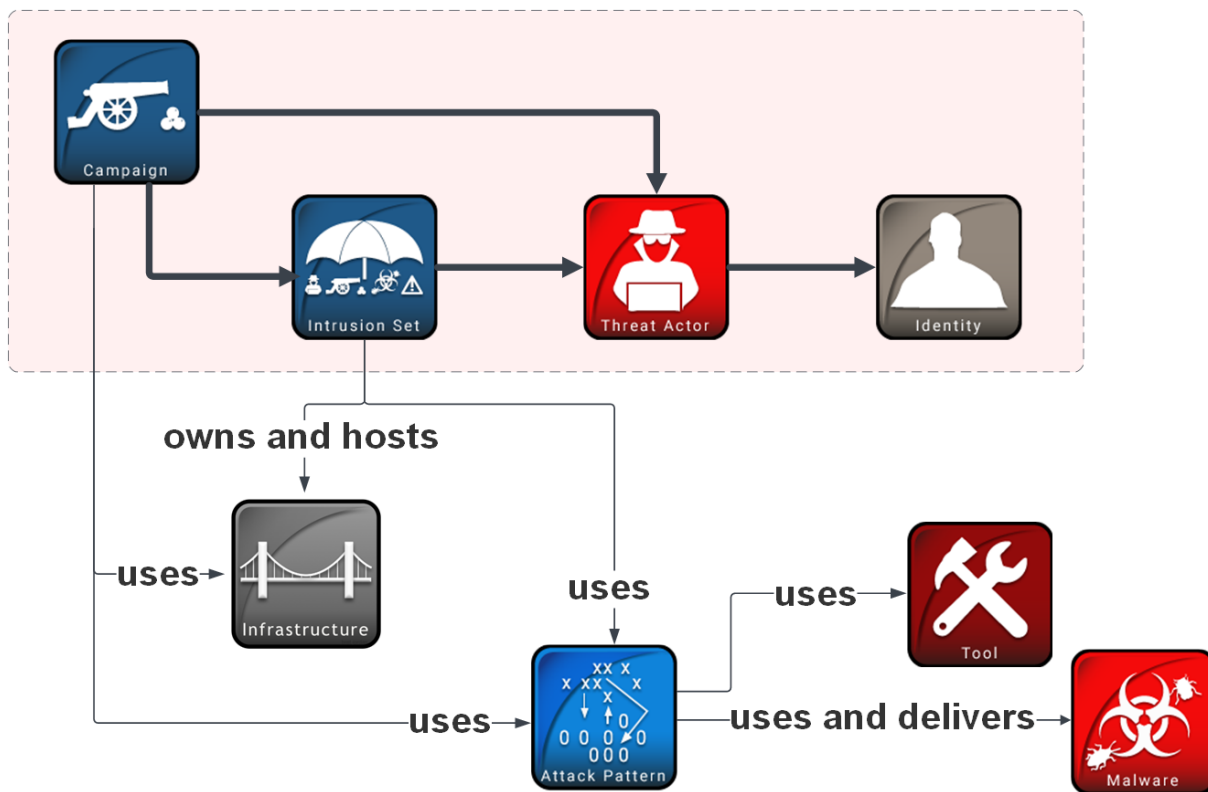
Figure 1. Attributed-to relationships in STIX 2 are shown with the arrows in bold (the icons are taken from https://github.com/MISP/intelligence-icons , accessed on 21 January 2024).
