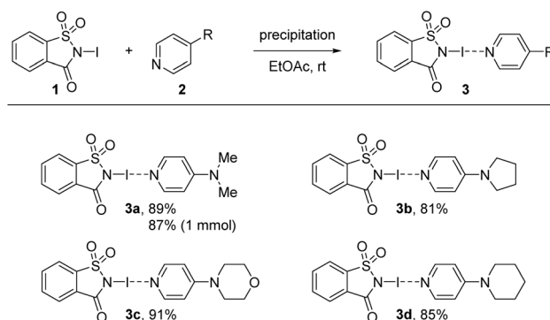
Scheme 2 Synthesis of XB complexes 3 in the reaction between NISac ( 1 ) and 4-substituted pyridine derivatives 2 by precipitation. All reactions were performed on a 0.32 mmol scale. NISac (1, 100 mg, 0.32 mmol, 1.0 equiv.), pyridine derivative 2 (0.32 mmol, 1.0 equiv.), both dissolved in 1.5 mL EtOAc, then combined. The XB complexes 3a–3d were isolated by filtration.
