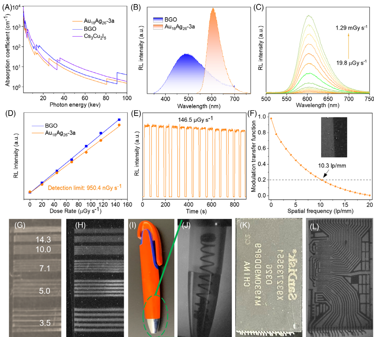
FIGURE 3 The radioluminescence properties of \text{Au}_{18}\text{Ag}_{26}\text{-3a} nanocluster. (A) X-ray absorption spectra of \text{Au}_{18}\text{Ag}_{26}\text{-3a} , \text{Bi}_4\text{Ge}_3\text{O}_{12} (BGO), and \text{Cs}_3\text{Cu}_2\text{I}_5 measured as a function of the irradiation energy. (B) RL spectra of \text{Au}_{18}\text{Ag}_{26}\text{-3a} and BGO at the optimal thickness (dose rate, 146.5 \mu\text{Gy s}^{-1} ). (C) Dose rate-dependent RL spectra of \text{Au}_{18}\text{Ag}_{26}\text{-3a} over the dose rate range of 19.8 \mu\text{Gy s}^{-1} to 1.29 \text{ mGy s}^{-1} . (D) Detection limits of \text{Au}_{18}\text{Ag}_{26}\text{-3a} and BGO. (E) The RL stability of \text{Au}_{18}\text{Ag}_{26}\text{-3a} under continuous X-ray irradiation (dose rate, 146.5 \mu\text{Gy s}^{-1} ). (F) Modulation transfer function (MTF) of the \text{Au}_{18}\text{Ag}_{26}\text{-3a} -PMMA film, measured by the slanted-edge method (inset). (G and H) The optical (G) and X-ray photographs (H) of a standard X-ray resolution pattern plate (lp/mm). (I and J) Photographs of a ball pen with a metal spring inside before (I) and after (J) X-ray exposure. (K and L) Photographs of an electronic chip before (K) and after (L) X-ray exposure.
