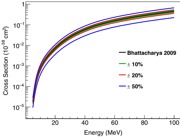
FIG. 10. \nu_e - {}^{40}\text{Ar} cross section versus energy with various scaling factors applied. Reference [31] provided the cross-section model using nuclear matrix element data from Ref. [49].
