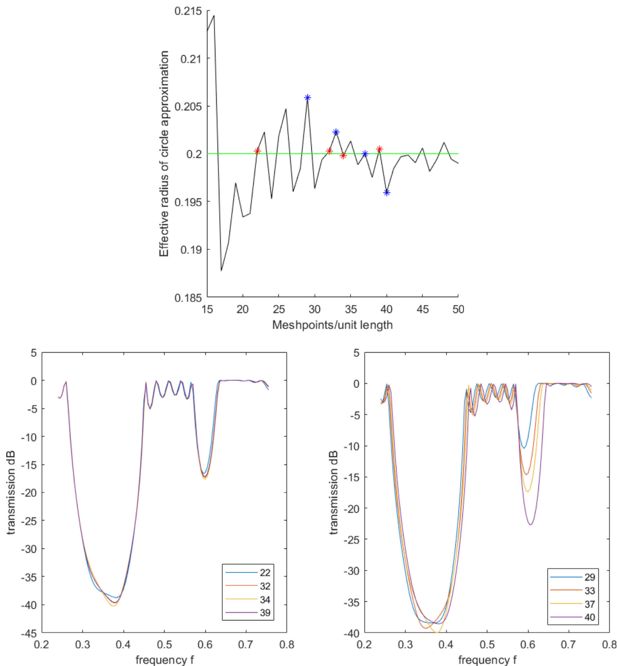
FIGURE 9 Approximating the circular cross-sections of a dielectric rod with rectangles, the accuracy of the approximation and simulation results depend strongly on the number of mesh points per unit length.
