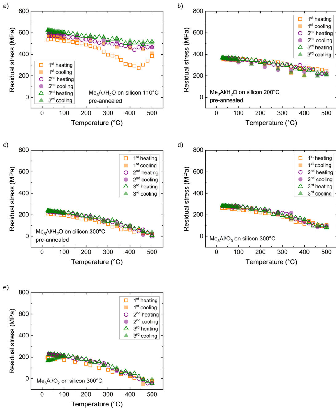
FIG. 2. Residual stress as a function of thermal cycling temperature for ALD Al 2 O 3 on silicon from Me 3 Al and H 2 O grown at (a) 110, (b) 200, and (c) 300 °C and (d) from Me 3 Al and O 3 grown at 300 °C and (e) Me 3 Al and O 2 (plasma) grown at 300 °C.
