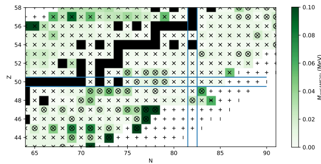
Fig. 3: In this figure we plot in a color-coded neutron vs proton number plane ( N - Z plane) the 1\sigma error of the mass-excess values reported in AME20. With black we label stable nuclei. In addition, we label with ( x ) measured masses in AME20, with ( + ) extrapolated masses which are both in AME16 and AME20 and with ( I ) extrapolated masses that are reported only in AME20. We circle the elements that are accessible for Penning traps and for which the mass measurements can drastically reduce the error bar. Vertical and horizontal lines label the N=82 closed neutron and Z=50 proton shell respectively.
