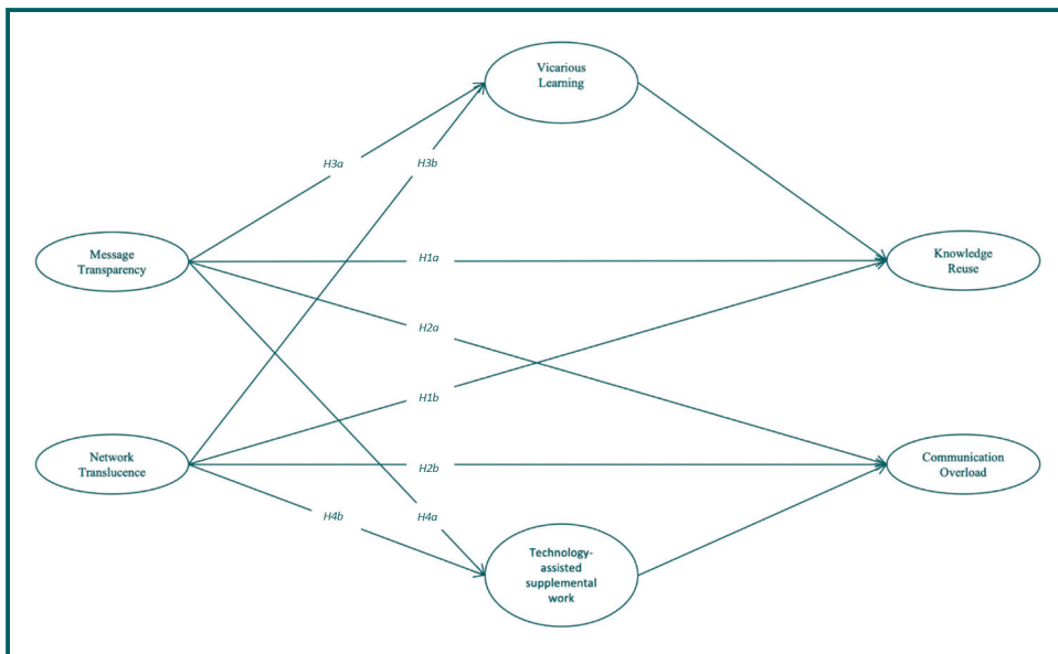
Figure 1 Hypothesized model
