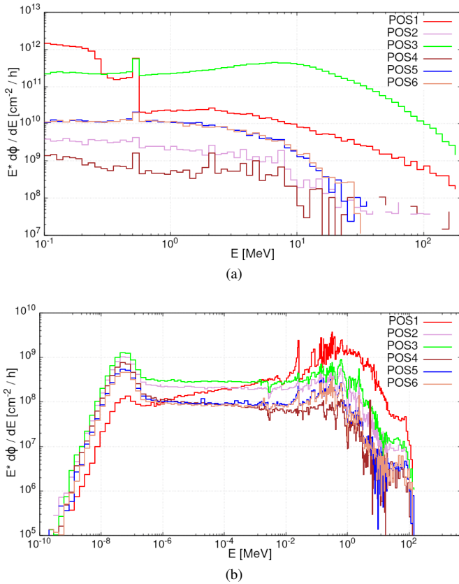
Fig. 6. Simulated distributions of photons (a) and neutrons (b) per unit lethargy in the reference test positions at CLEAR.
