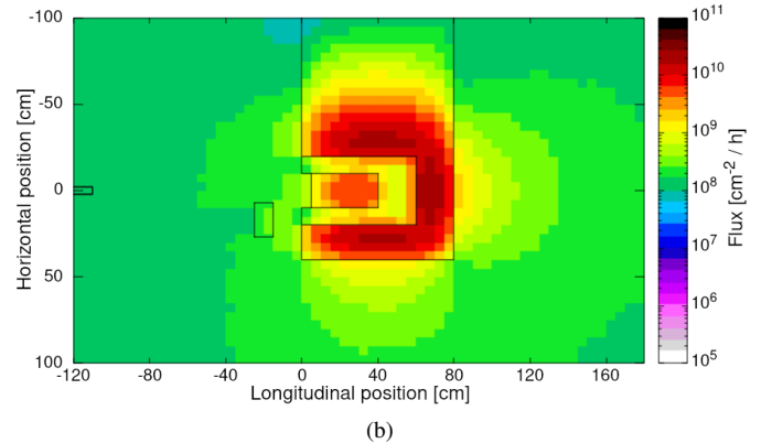
Fig. 9. Top view of ISSI HEH-eq flux (a) and thermal neutron equivalent flux (b) at beam height.
