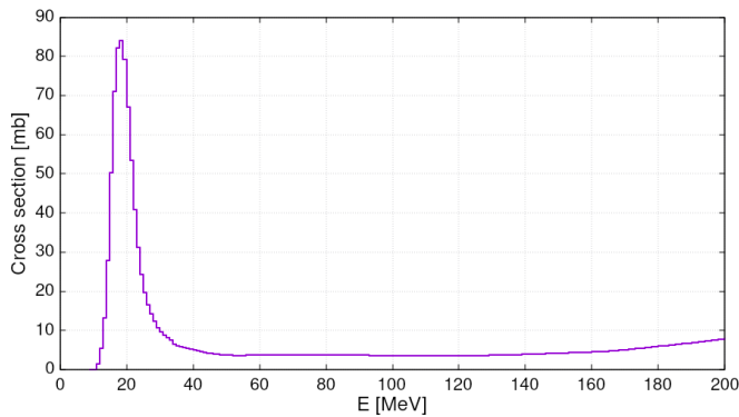
Fig. 3. Total cross section of photonuclear reactions in Fe as a function of photon energy.
