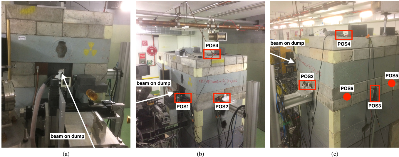
Fig. 1. Front (a), side (b) and back (c) views of the CLEAR THz test station and beam dump, showing the beam axis and the reference test positions where SEU measurements have been taken.
