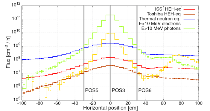
Fig. 12. Flux profiles vs horizontal position behind the CLEAR dump.
