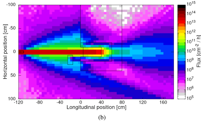
Fig. 10. Top view of E > 10 MeV photon (a) and electron (b) fluxes at beam height.
