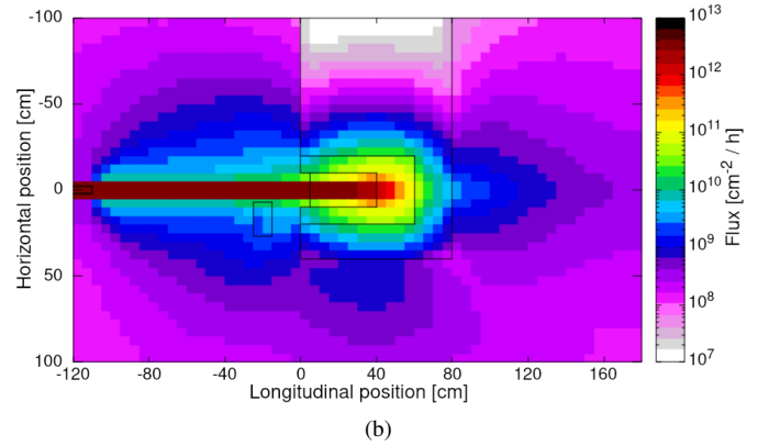
Fig. 11. Top view of TID (a) and Silicon 1-MeV neutron equivalent flux (b) at beam height.
