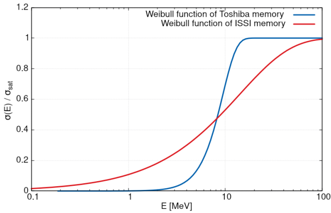
Fig. 8. Weibull functions of the Toshiba and ISSI memories, obtained through Equation 1 with the parameters in Table II.
