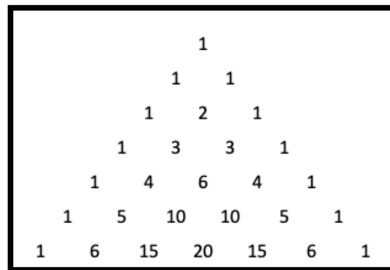
Figure 1. Pascal's triangle.
