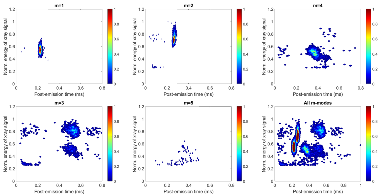
FIG. 13. The dependence of post-emission time on the energy emitted per burst mode m . The data corresponds to a B_{\min}/B_{ecr} value of 0.76, neutral gas pressure of 3.5 \times 10^{-7} mbar, and RF power of 400 W. The x-ray energy is normalized to the maximum value corresponding to all burst modes m combined. The plot shows individually each mode m = 1, \dots, 5 and a combined plot of all m -modes. The false color represents the data point density, with blue representing the lowest.
