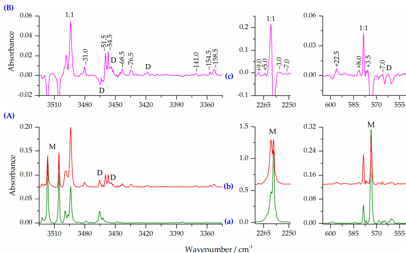
Figure 5. (A) The \nu_{\text{NH}} , \nu_{\text{asNCO}} and \delta_{\text{NCO}} regions in the spectra of matrices: HNCO/N 2 /Ar = 1/4/5600 (a), and matrix after 10 min at 33 K/10 K (b); (B) the difference spectrum (c) obtained by subtracting the spectrum (a) from the spectrum (b) (pink trace). Letters M and D denote the HNCO monomer and dimer bands, respectively.
