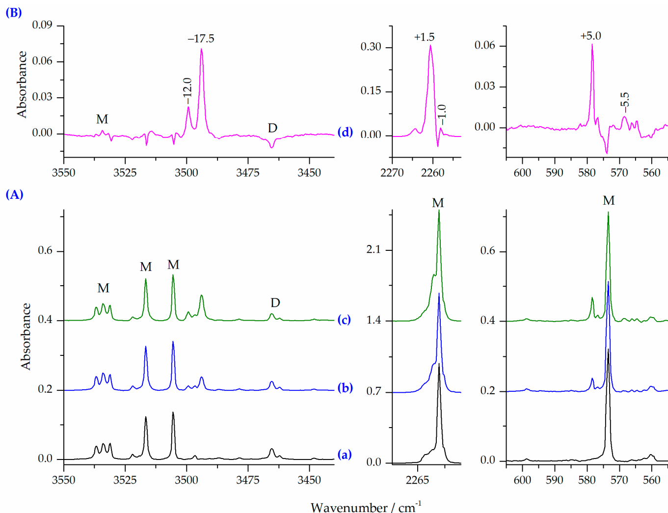
Figure 4. (A) The \nu_{\text{NH}} , \nu_{\text{asNCO}} and \delta\text{NCO} regions in the spectra of matrices: \text{HNCO}/\text{Ar} = 1/6000 (a), \text{HNCO}/\text{N}_2/\text{Ar} = 1/2/5600 (b), \text{HNCO}/\text{N}_2/\text{Ar} = 1/4/5600 (c); (B) the difference spectrum (d) obtained by subtracting the spectrum (a) from the spectrum (c) (pink trace). Letters M and D denote the HNCO monomer and dimer bands, respectively.
