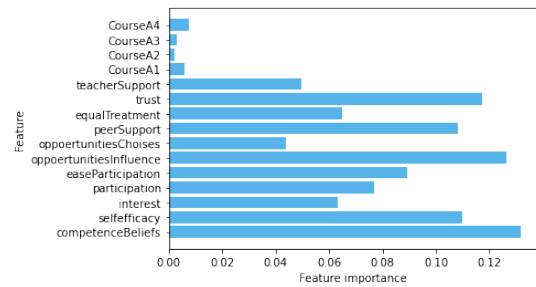
FIGURE 10. Feature importances of the random forest model predicting the agency profile. For the random forest, the agency dimensions are more important than the course features.
