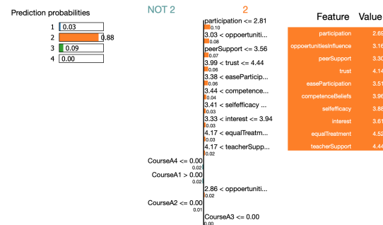
FIGURE 11. LIME rules explaining why the random forest model predicted an agency profile PAP2 student from the test set to be profile PAP2 (i.e., a true positive) with the highest probability. The most important local explanation why this student was assigned to this profile are his/her participation values.
