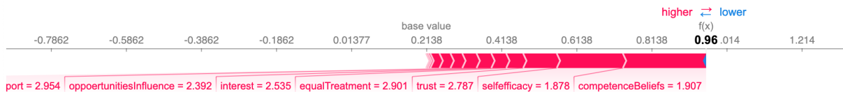
FIGURE 7. SHAP values explaining why the random forest model predicted an agency profile PAP1 student studying in course A3 from the test set to be profile PAP1 (true positive). The most important explanations are the low competence beliefs and self-efficacy values of this student.
