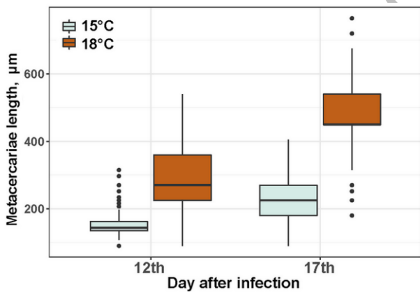
Fig. 2. The difference in metacercariae sizes at different temperatures. ‘Boxes’ represent a median with the interquartile range (IQR), whiskers extend from the highest to lower values within 1.5 \times \text{IQR} .
