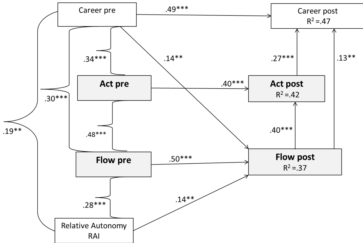
Figure 4: The final path model.
