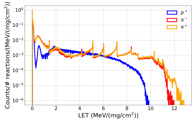
Fig. 13. Yield of secondary ions normalized to the number of interactions as a function of their LET for mono-energetic protons, negative pions and positive pions at 21 MeV.
