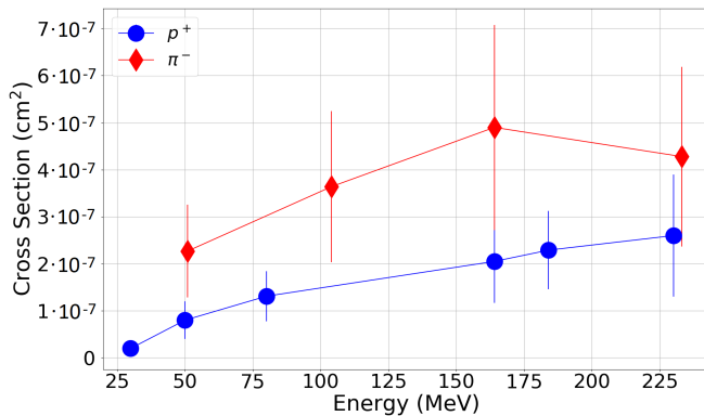
Fig. 1. Negative pion and proton SEL cross-sections for the Brilliance SRAM with 95% confidence level error bars [5].
