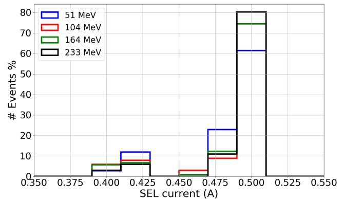
Fig. 3. Histograms of the distribution of high-state currents due to pion interactions of the tested energies for the Brilliance SRAM. The red bin is underneath the green bin for 0.5 A.
