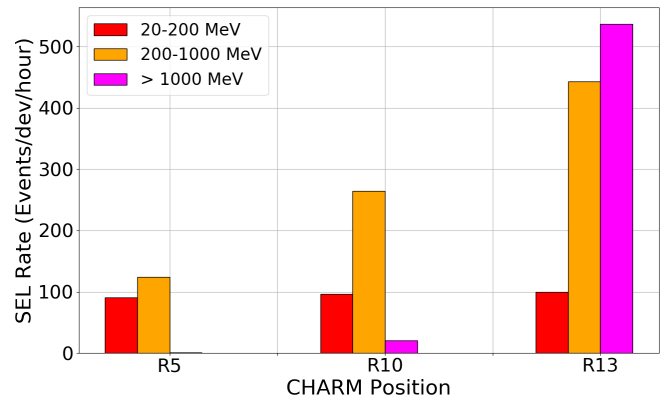
Fig. 17. SEL rates from pions from three energy ranges and three CHARM positions.
