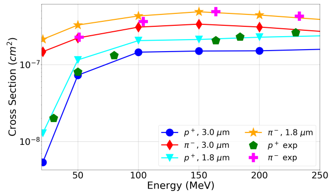
Fig. 5. Proton and negative pion SEL cross-sections simulated with FLUKA for a SV thickness of 3.0 and 1.8 \mu\text{m} and compared to the Brilliance experimental data.
