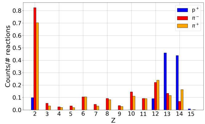
Fig. 9. Yield of secondary ions produced by nuclear reactions as a function of their atomic number normalized to the number of interactions for mono-energetic protons, negative pions and positive pions at 21 MeV.
