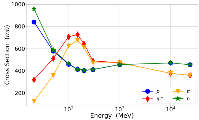
Fig. 7. Nuclear reaction cross-section in millibarns ( 1 \text{ mb} = 10^{-27} \text{ cm}^2 ) of protons, neutrons, negative pions and positive pions when interacting with Silicon nuclei as a function of energy. For pions, this includes inelastic scattering and absorption.
