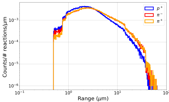
Fig. 15. Yield of secondary ions normalized to the number of interactions as a function of their range for mono-energetic protons, negative pions and positive pions at 200 MeV.
