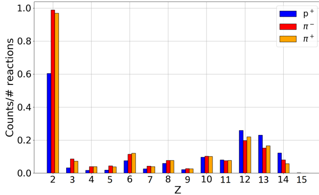
Fig. 8. Yield of secondary ions produced by nuclear reactions as a function of their atomic number normalized to the number of interactions for mono-energetic protons, negative pions and positive pions at 200 MeV.
