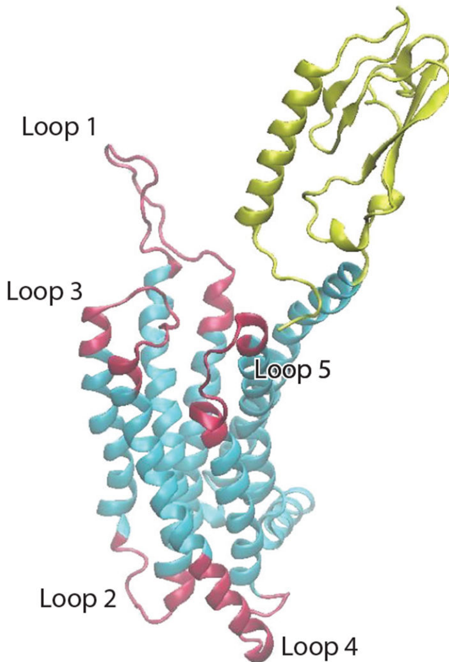
Figure 4. The graphic representation of the GLP-1R (glucagon-like peptide-1 receptor). The red loops are accelerated by temperature-accelerated molecular dynamics. In addition to the loops, the mass center of the extracellular domain (ECD) is accelerated ( yellow region ), the intracellular domain (ICD) is the lower part of the protein in the vicinity of and including loops 2 and 4, and the transverse membrane domain lies between the ECD and ICD. The lipid membrane, water, and salt ions are not rendered for clarity.
