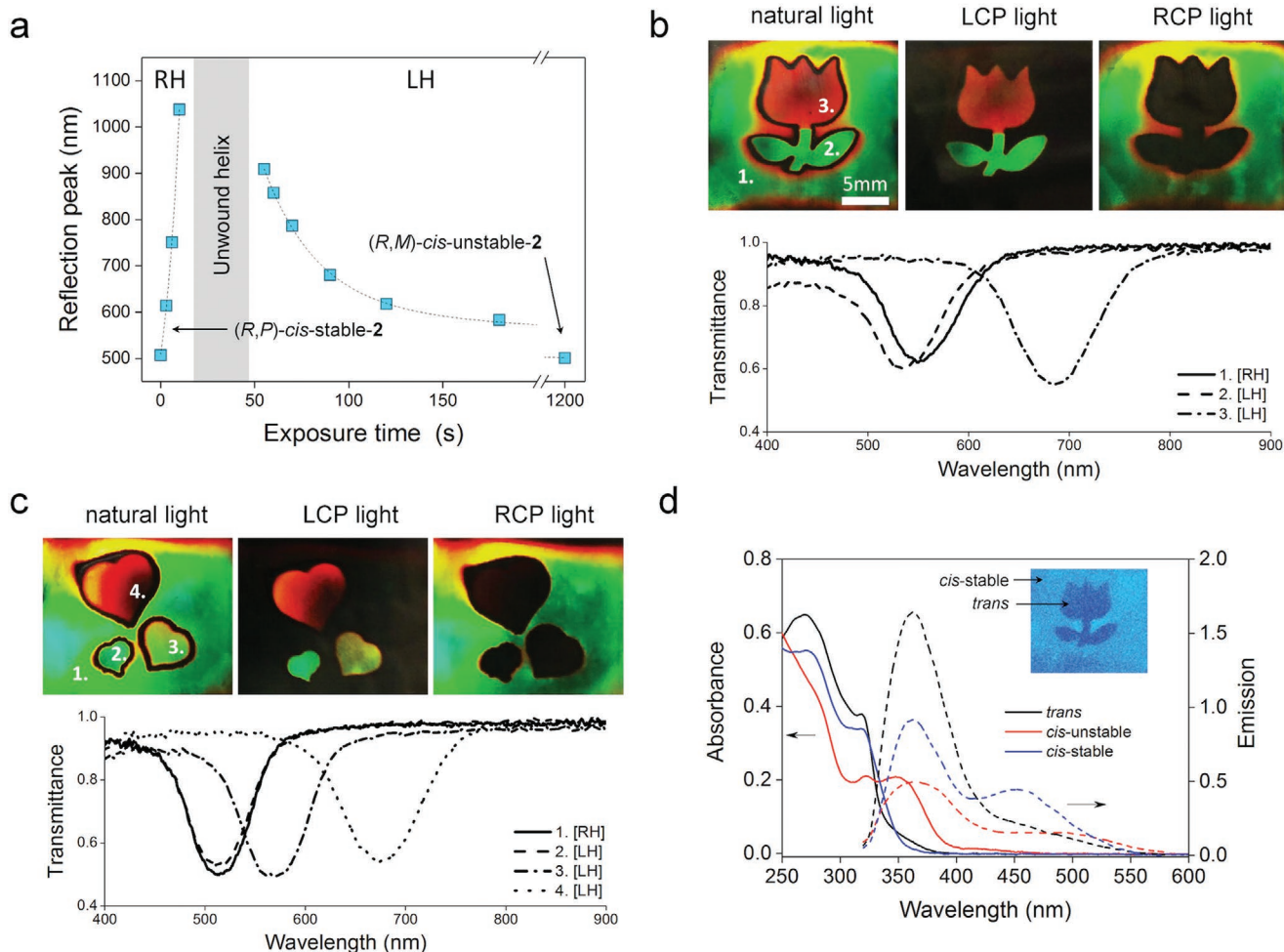
Figure 4. Photopatterning multiple and circularly polarized reflection colors in a single material. a) Evolution of helix pitch and handedness of a liquid crystal (ZLI-1132) doped with motor cis -stable-2 (4 wt%) upon exposure to UV light ( \lambda = 300 nm). The notations RH and LH indicate right- and left-handed cholesteric helices, respectively. b,c) The thin cholesteric layers with recorded patterns were visualized under natural (nonpolarized) light and under left- and right-circular polarized light (LCP and RCP, respectively). Samples were irradiated at \lambda = 300 nm, through a mask. The reflection from the cholesteric liquid crystal can be visualized selectively by using circular polarizers, while irradiating with natural (nonpolarized) light allows visualizing of both RH and LH reflection colors. The transmission spectra corresponding to the different colors are provided in the panel below. d) Absorbance (solid lines) and fluorescence (dashed lines) spectra of liquid crystal film (ZLI-1695) doped with motor cis -stable-2 (1 wt%). The inset shows a fluorescence image for irradiation through a mask with \lambda = 365 nm light (the excitation wavelength being \lambda = 312 nm). The motor is in the trans -state inside the flower pattern, while the outside of the flower pattern is in the cis -stable state. These two areas are distinguishable by their fluorescence. The dimension of the sample is 2 \times 2 cm.
