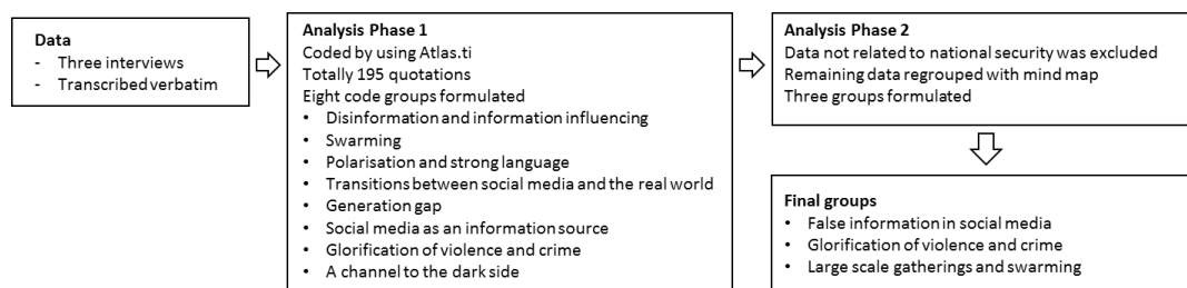
Figure 1: Analysis process
