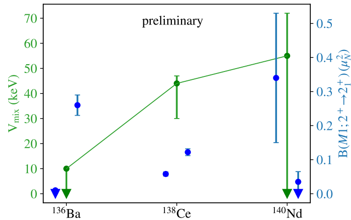
Figure 6. The M1 transition strengths B(M1; 2_1^+ \rightarrow 2_1^+) of the fragments of the 2_{1,ms}^+ state of N = 80 isotones are shown in blue. The resulting F -spin mixing matrix elements are shown in green.
