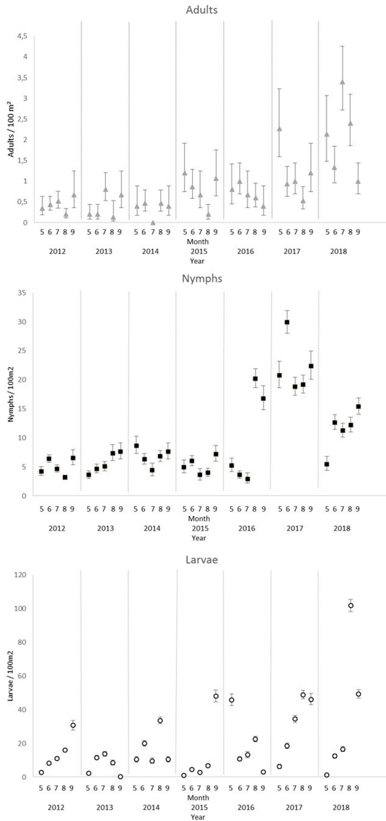
Fig. 5. Seasonal patterns of adult, nymph and larvae I. ricinus activity on Seili Island (with 95% CL). Information on statistically significant differences between specific months and years are available from the authors on request.
