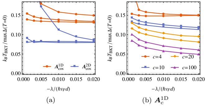
Figure 12. Behavior of the Berezinskii–Kosterlitz–Thouless transition temperature T_{\text{BKKT}} at optimal doping \mu = \mu_{\text{opt}} . The ratio k_{\text{B}}T_{\text{BKKT}}/\max\Delta(T=0) for (a) the cosine potentials and (b) \mathcal{A}_c^{\text{1D}} with varying c . In (a) both potentials have three curves corresponding to \beta = 20, 30, 40 (1D potential) or \beta = 10, 15, 20 (2D potential), from top to bottom in the flat-band regime, while in (b) each c has two curves corresponding to \beta = 30, 40 , from top to bottom. In the flat-band regime the ratio tends approximately to a constant depending slightly on the potential, as in (35).
