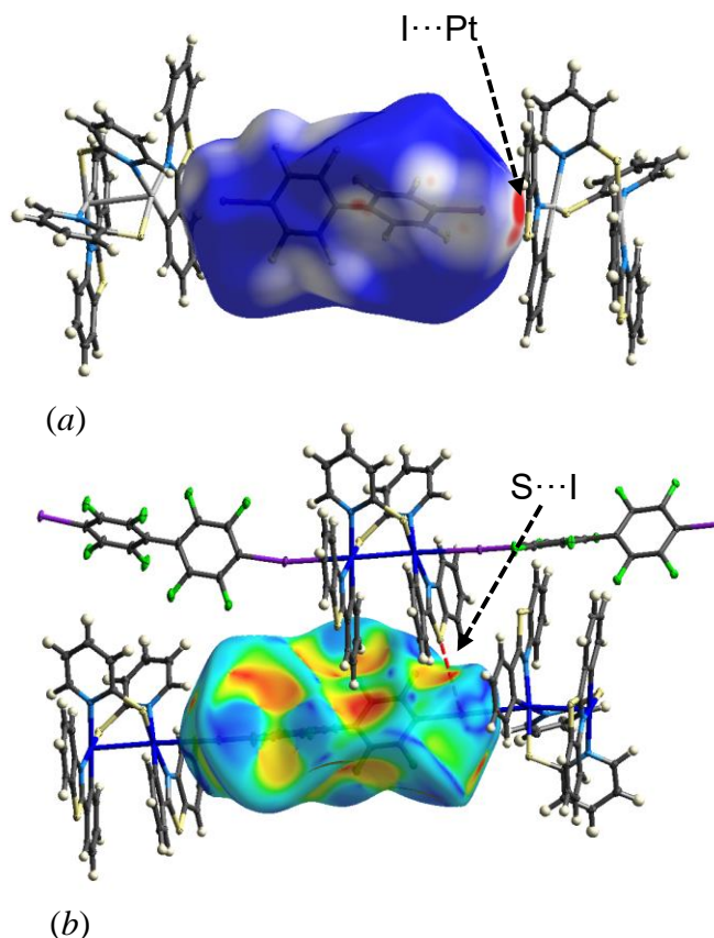
Figure 11. The Hirshfeld surfaces for [1\cdot 1,1'\text{-FIDB}]_n . (a) mapped with d_{\text{norm}} over the range – 0.20 (red) to 1.00 (blue); (b) shape index (S), mapped from –1.0 (concave hollows; red) → 0.0 (minimal saddle; green) → +1.0 (convex bumps; blue).
