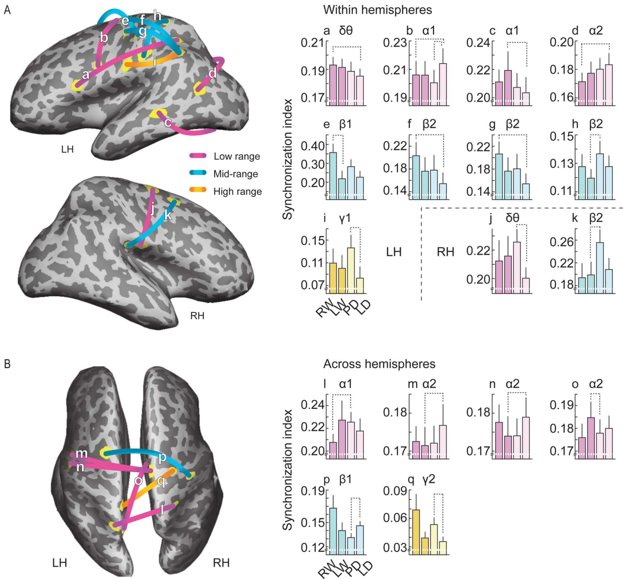
Figure 5. Task-sensitive corticocortical phase synchronization in the left and right hemispheres (A) and across the hemispheres (B). The cortical surface view illustrates the corticocortical connections (a–q), which showed modulated phase synchrony for the different variants of handwriting task (Fig. 1C). Color-coding refers to the spectral ranges. The bar graphs (below) show SI values ( \pm SEM) for each connection. Task contrast ( n = 10 ; maximum-statistics permutation testing based on t-statistics, 95% threshold) and the frequency band of the effect are indicated. Note the different ranges of y-axis values and the fact that permutation testing can highlight statistical differences that do not fully comply with the apparent differences in mean SI levels (see, e.g., connections p and q).
