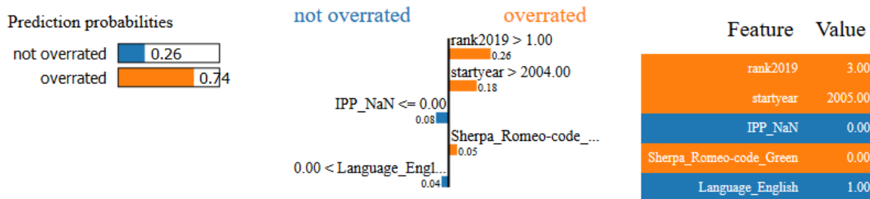
Fig. 3. Five most important LIME explanations of the gradient boosting classifiers predicting if the rank of a publication channel is overrated for the International Journal of Education through Art . The high current rank, the young age of the journal (start year 2005), and the green sherpa code were the most important local explanations classifying the channel as overrated (which it is). However, the language of the publication channel (English) and the fact that the IPP is available (not missing) were reasons for the model to classify this publication channel with some probability as not overrated.
