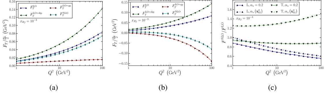
Figure 1: (a): F_T(Q^2) LO and NLO contributions in the "unsubtracted" scheme. (b): F_T(Q^2) in the approximative x_{Bj} -subtracted scheme. (c): Ratios F^{NLO}(Q^2)/F^{LO}(Q^2) with fixed and running coupling.
