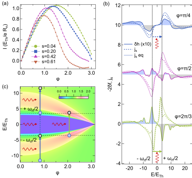
FIG. 3. (a) Calculated current-phase relation for different reduced power s . Calculation parameters are \hbar\omega_{rf}/E_{Th} = 7 , \Gamma/E_{Th} = 0.4 , k_B T/E_{Th} = 7 , and \Delta/E_{Th} = 55 . (b) Calculated equilibrium j_{s,eq} and nonequilibrium j_s spectral currents and modifications of the distribution function -2\delta f for different phases. Calculation parameters are as in (a). Full (dashed) horizontal arrows represent the high (low) probability interband transitions. (c) Color-coded sketch of the normalized energy-phase dependent density of states of a long diffusive SNS junction. Full (dashed) vertical arrows represent the high (low) probability inelastic transitions. Gray (blue) circles represent electronlike (holelike) quasiparticles.
