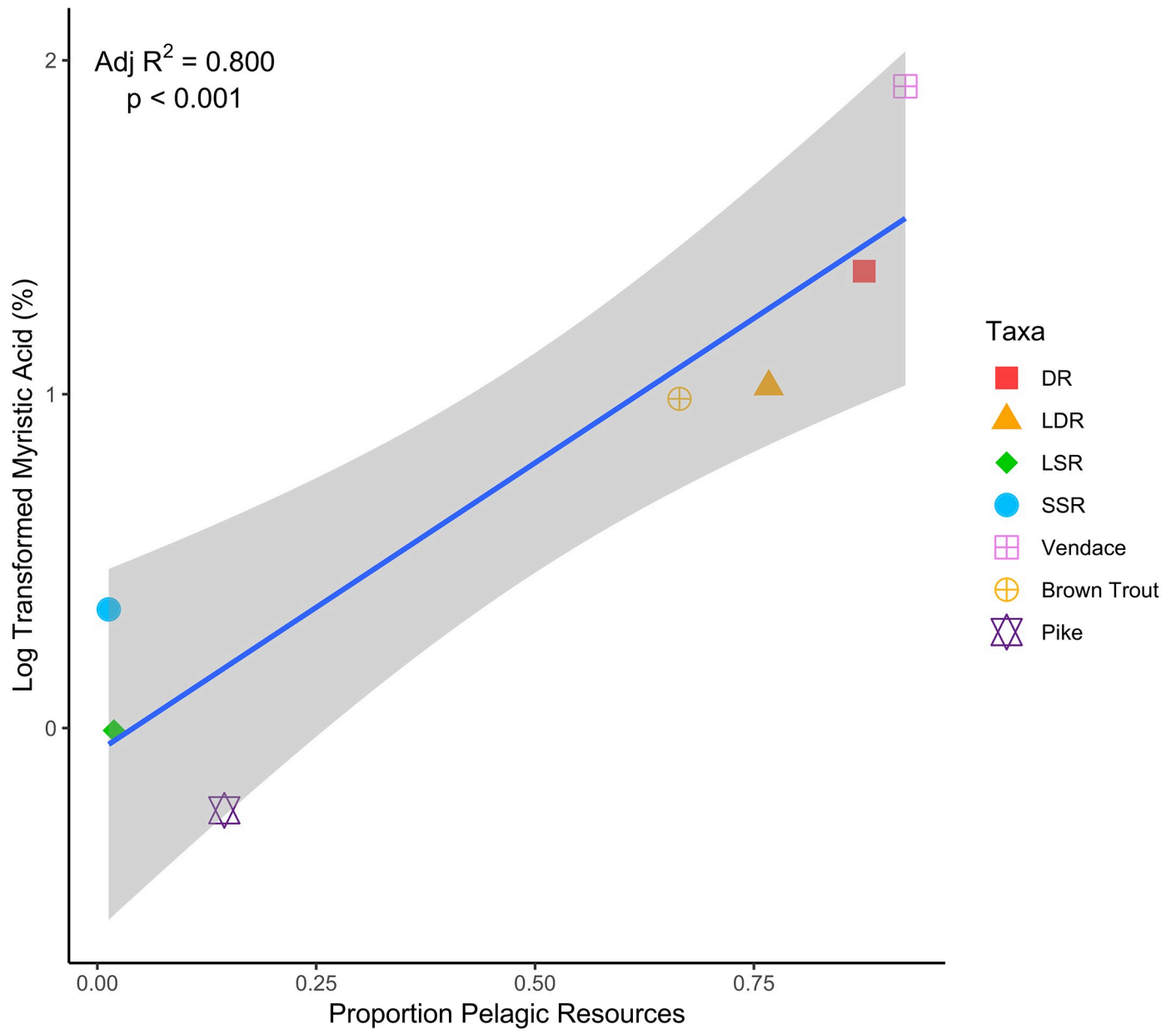
Fig 5. Relationship between log-transformed myristic acid concentration (%) and mean pelagic reliance (estimated from SIAR model based on \delta^{13}\text{C} , \delta^{15}\text{N} and diet data) across all fish taxa. DR = densely-rakered whitefish, LDR = large densely-rakered whitefish, LSR = large sparsely-rakered whitefish, SSR = small sparsely-rakered whitefish.
