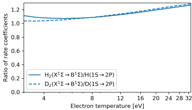
FIG. 4. Ratio of electron impact excitation rate coefficients to the lowest excited states of the atom ( 1S \rightarrow 2P ) and molecule ( X^1\Sigma_g^+ \rightarrow B^1\Sigma_u^+ ) for hydrogen and deuterium as a function of Maxwellian electron temperature at T_{\text{vib}} = 5000 K (Boltzmann distribution). The cross sections are from Refs. 12 and 16.
