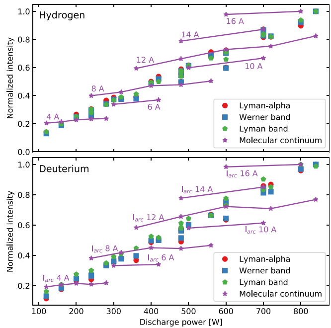
FIG. 7. The VUV emission as a function of the arc discharge power in different emission bands at 0.4 Pa neutral gas pressure. The data are normalized to the maximum intensity observed during the parameter sweep.
