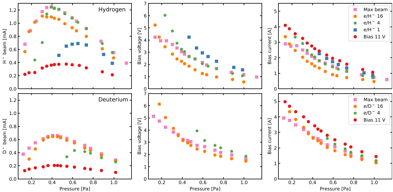
FIG. 10. Measured H^- currents and biased plasma electrode parameters as a function of neutral gas pressure for different H^-/e^- ratios at 70 V arc voltage and 12 A arc current (840 W).
