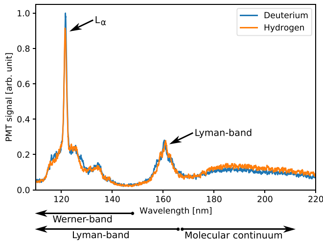
FIG. 6. The measured VUV spectra from hydrogen and deuterium plasmas. The spectra are measured at 0.5 Pa and 840 W arc discharge power (12 A, 70 V). The spectra are not corrected for spectral transmittance.
