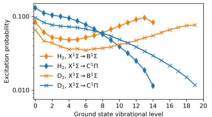
FIG. 3. Vibrational excitation distribution on the electronic ground state resulting from the hydrogen and deuterium molecule excitations to B^1\Sigma_u^+ and C^1\Pi_u states at T_{vib} = 5000 \text{ K} (Boltzmann distribution). The excitation probabilities are calculated using cross sections from Ref. 16 and Franck-Condon coefficients from Ref. 14.
