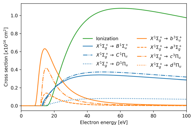
FIG. 1. Electron impact cross sections for the most significant inelastic collision processes of hydrogen molecules at electron energies above 10 eV. Ionization, singlet excitation, and triplet excitation cross sections are marked with green, blue and orange colors, respectively. The cross sections are from Ref. 12.
