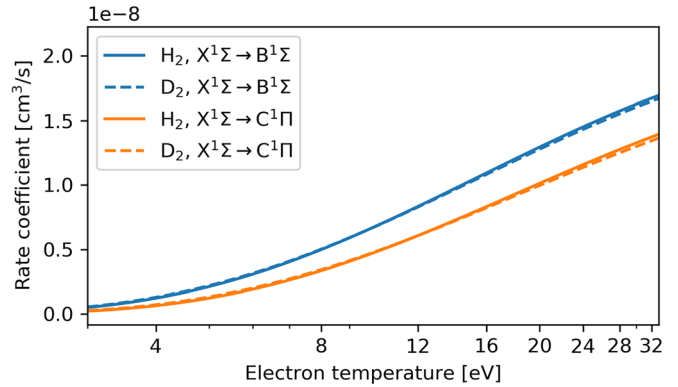
FIG. 2. Hydrogen and deuterium rate coefficients to B^1\Sigma_u^+ and C^1\Pi_u states as a function of the Maxwellian electron temperature at T_{vib} = 5000 \text{ K} (Boltzmann distribution). The cross sections are from Ref. 16.
