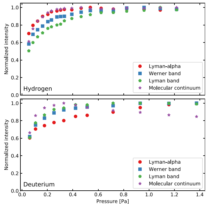
FIG. 8. The VUV emission as a function of neutral gas pressure in different emission bands at 70 V arc voltage and 12 A arc current (840 W). The data are normalized to the maximum intensity observed during the parameter sweep.
