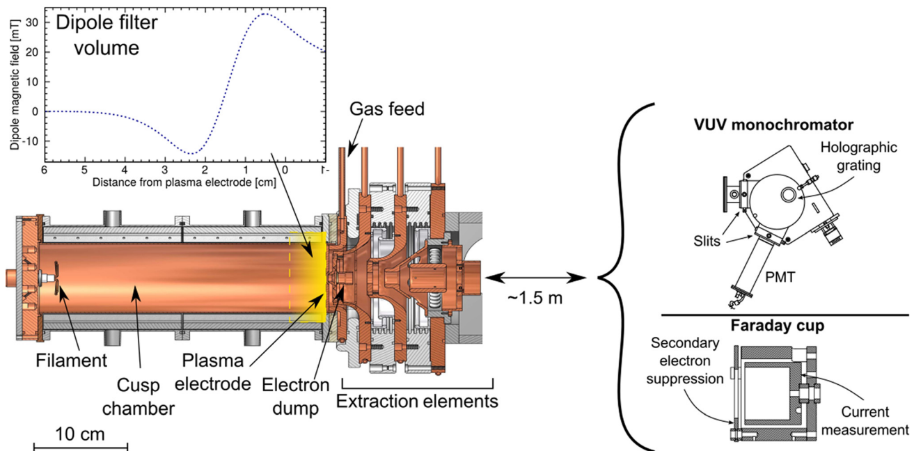
FIG. 5. The experimental setup. The negative and positive bias voltages of the filament and the plasma electrode, both referenced to the plasma chamber, i.e., ion source potential, are generated by 70 V/12 A and 20 V/10 A power supplies, respectively. The nominal extraction element voltages are as follows (from left to right): source potential, -5.9 kV; extraction (puller) electrode housing the electron dump, 1 kV; and first electrostatic Einzel lens, 1.5 kV, referenced to the (negative) ion source potential; and intermediate accelerating electrode, 2 kV; second Einzel lens, 2.3 kV; and third Einzel lens, 10.5 kV, referenced to the laboratory ground.
