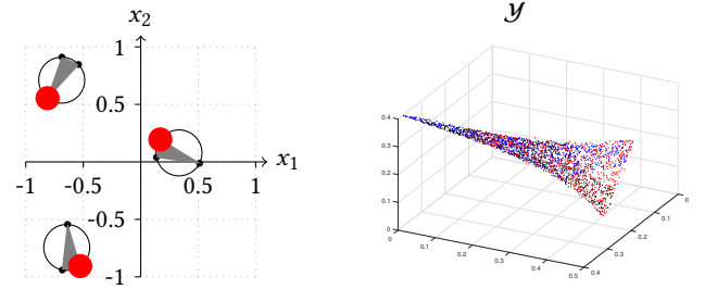
Figure 7: Illustrations of penalty locations generating non-identical disconnected Pareto sets. Left : Penalty regions intersect the three regions \mathcal{R}_i in different areas. Right : \mathcal{X} is sampled and evaluated under \mathbf{f} , the non-dominated subset is shown, with the three colours represented in the three different regions \mathcal{R}_j responsible for the front members.
