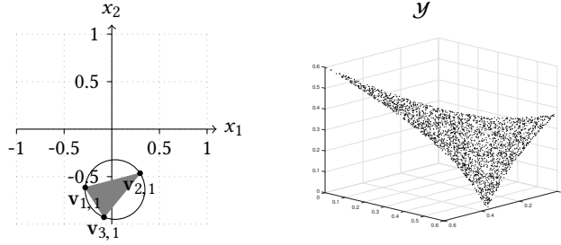
Figure 1: A problem with three objectives, V_k = \{v_{k,i}\} , |V_k| = 1 . Left: The three locations in X , which lie on the circumference of the black circle, determine the objective value minima. They describe a three-sided polygonal Pareto set (coloured grey). Right: Samples on the corresponding Pareto front generated by Monte Carlo sampling the Pareto set.
