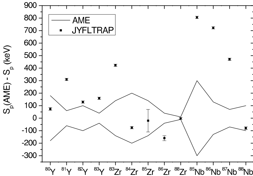
Fig. 9. Proton separation energies for the measured nuclides relative to AME values. The two lines show the corridor of uncertainties taken from ref. [14]. The mass of the (Z-1, N) nucleus is from this experiment for ^{83}\text{Zr} , ^{84}\text{Zr} , ^{85}\text{Nb} , ^{86}\text{Nb} and ^{87}\text{Nb} . For the others, the AME mass [14] of the (Z-1, N) nucleus has been used.
