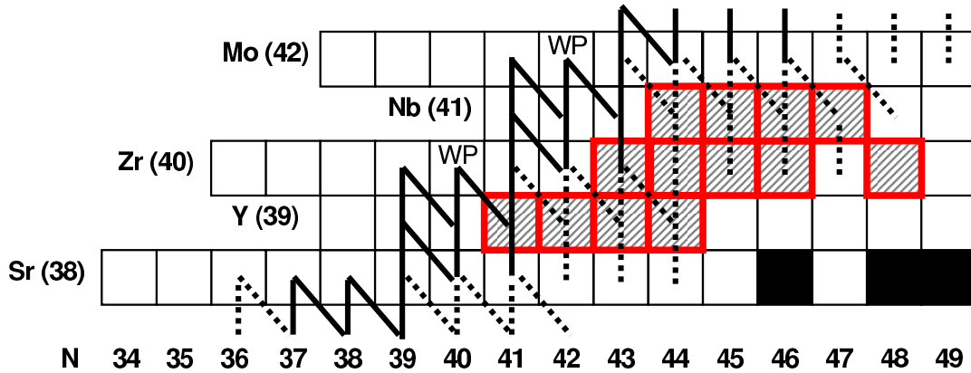
Fig. 1. The rp process path in the region close to A = 80 for steady state burning [3]. The reaction flows of more than 10 % are shown by a solid line and of 1–10 % by a dashed line. The studied nuclides are highlighted by squares. Waiting-point nuclei ^{80}\text{Zr} and ^{84}\text{Mo} are labeled as WP.
