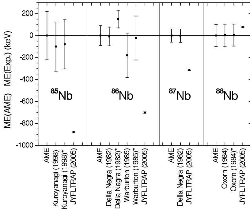
Fig. 8. Mass excesses of the measured Nb isotopes relative to AME values [14]. The error bars represent only the uncertainties of the corresponding experiments. The labels refer to beta-decay experiments of Kuroyanagi et al. [29], Della Negra et al. [33], Warburton et al. [34] and Oxorn and Mark [37]. The values of 85,86,88 Nb marked with an asterisk have been calculated with the mass excesses of the corresponding daughter nuclei 85,86,88 Zr measured in this experiment at the JYFLTRAP. The other mass excesses have been calculated with AME values for daughter nuclides.
