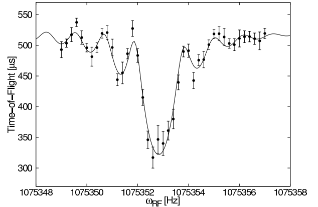
Fig. 4. Time-of-flight resonance of ^{84}\text{Zr} with an excitation time of 900 ms. The fit of the experimental data points is shown by a solid line.
