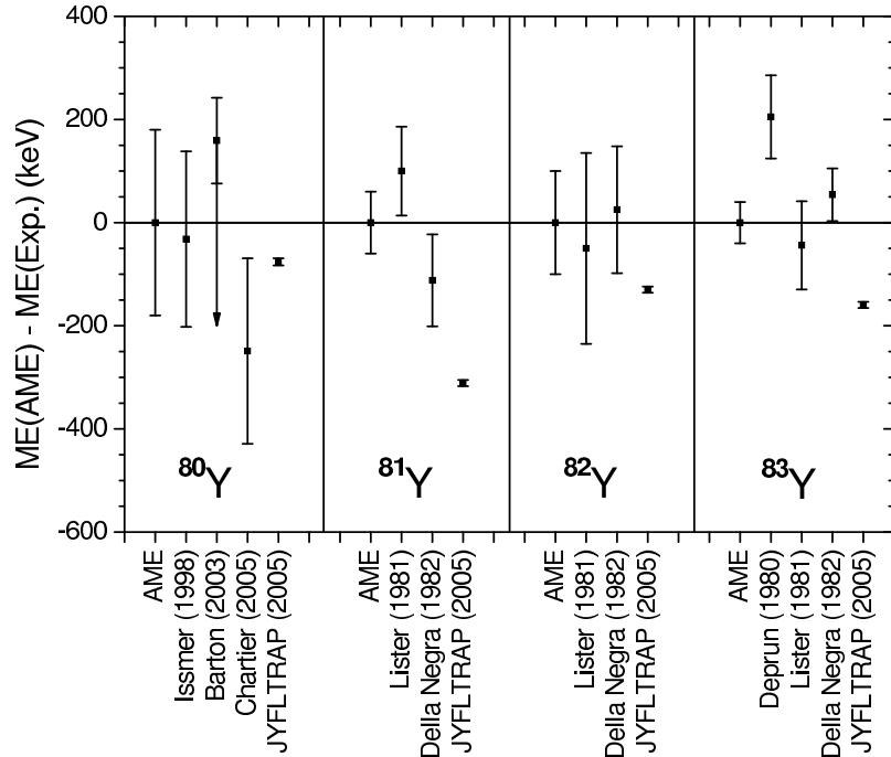
Fig. 6. Mass excesses of the measured Y isotopes relative to AME values [14]. The error bars represent only the uncertainties of the corresponding experiments. The labels refer to beta-decay experiments of Barton et al. [22], Lister et al. [18], Della Negra et al. [19], Deprun et al. [25] and to the TOF experiments at SARA by Issmer et al. [21] and at CSS2 by Chartier et al. [24]. The Q_{EC} value of ^{80}\text{Y} in [22] is only a lower limit which is indicated by an arrow in the figure.
