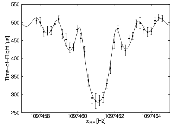
Fig. 5. Time-of-flight resonance of a reference nucleus ^{98}\text{Mo} with an excitation time of 900 ms. The fit of the experimental data points is shown by a solid line.
