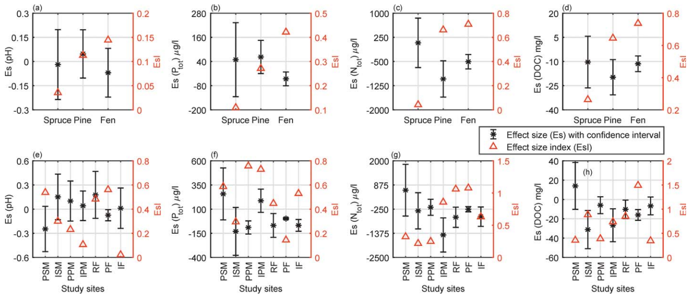
Figure 5. Mean restoration effect size ( Es ) and effect size index ( Esi ) of (a, e) pH level and (b, f) total phosphorus ( P_{tot} ), (c, g) total nitrogen ( N_{tot} ), and (d, h) dissolved organic carbon (DOC) concentration in pore water for different peatland classes (Figures 5a–5d) and trophic levels (Figures 5e–5h) regardless of time after restoration (bars show 95% confidence interval of Es ). PSM, poor spruce mires; ISM, intermediate spruce mires; PPM, poor pine mires; IPM, intermediate pine mires; RF, rich fens; PF, poor fens; and IF, intermediate fens.
