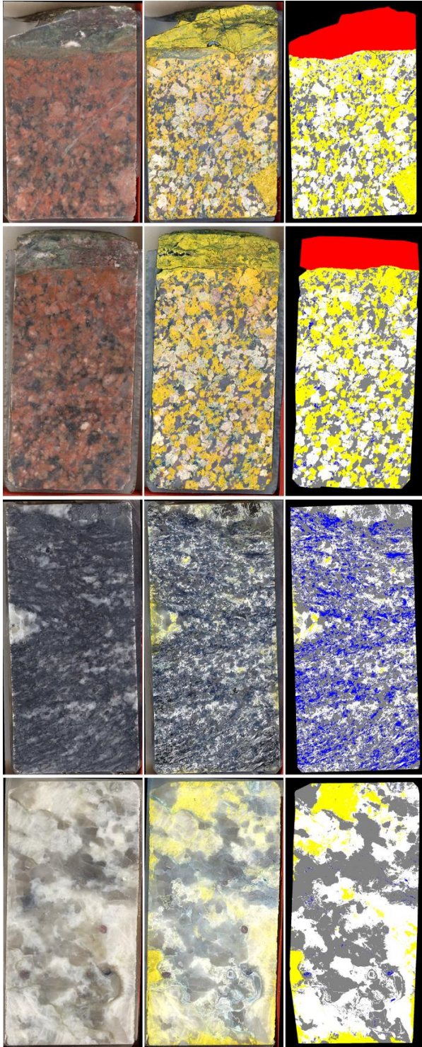
Fig. 3 The main minerals of LTDE-SD-GDR1 (1st row), LDTE-SD-GDR2 (2nd row), REPRO-VGN (3rd row) and REPRO-PGR (4th row) were stained chemically and segmented digitally. The photographs of original (left column) and chemically stained (middle column) of rock surface, and digitally segmented (right column) images are shown. In the stained and segmented images K-feldspar is yellow, plagioclase is white, mica minerals are blue, and quartz is gray. In the segmented images of LTDE-SD-GDR samples the alteration rim is shown as red. The width of the samples is 24 mm.
