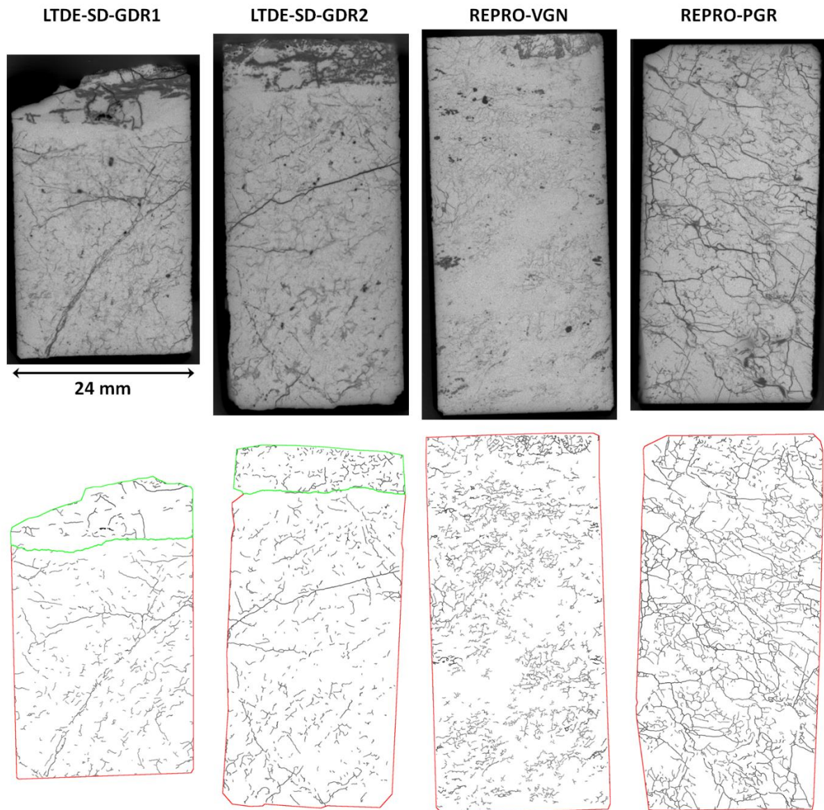
Fig. 4 The C-14-PMMA autoradiographs (upper panels) and segmented fractures and grain boundaries (lower panels) show the spatial porosity distribution of LTDE-SD-GDR1, LTDE-SD-GDR2, REPRO-VGN and REPRO-PGR samples (from left to right). In the C-14-PMMA autoradiographs dark shades of gray correspond to high porosity and light shades of gray to low porosity. In segmented fracture images red boxes indicate the analyzed area for the rock matrix and green boxes the analyzed areas for alteration rims.
