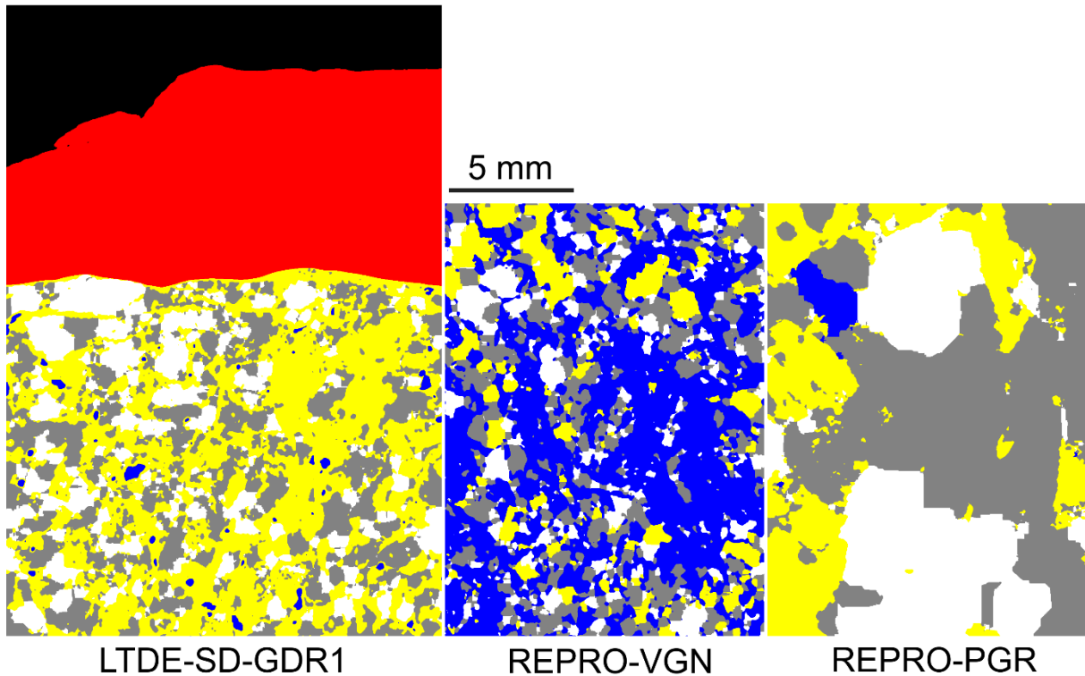
Fig. 9 The spatial distributions minerals of LTDE-SD-GDR1 (left), REPRO-VGN (middle) and REPRO-PGR (right). The result of grain segmentation and arbitrary division of mixed mineral phases show the partly artificial spatial distribution of mica minerals (blue), K-feldspar (yellow), quartz (gray), plagioclase (white) and alteration rim (red).
