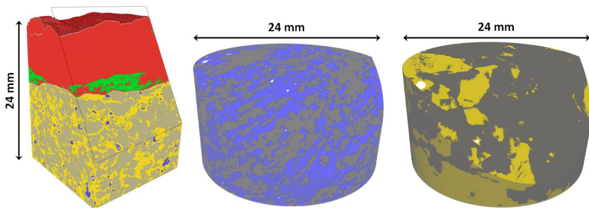
Fig. 8 The segmented tomographic images show spatial distribution of mica minerals (blue), K-feldspar (yellow), mineral phase (gray) that contain multiple minerals, alteration rim (red and green), and dense accessory minerals (white). In the LTDE-SD-GDR1 (left) and REPRO-PGR (right) samples the mineral phases contain mainly quartz and plagioclase, and in the REPRO-VGN sample (middle) K-feldspar, plagioclase and quartz.
