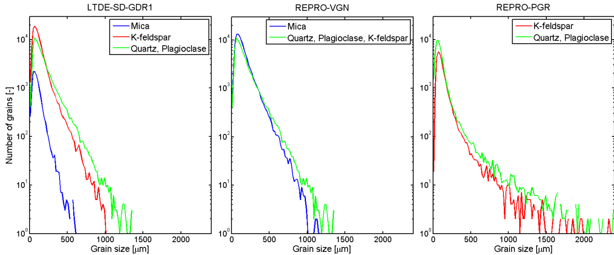
Fig. 7 Grain size distributions of the LTDE-SD-GDR1 (left column), REPRO-VGN (middle column), and REPRO-PGR (right column) samples. The distributions were determined from tomographic images with grains segmented, and the distributions are determined using 20 \mu\text{m} bin size.
