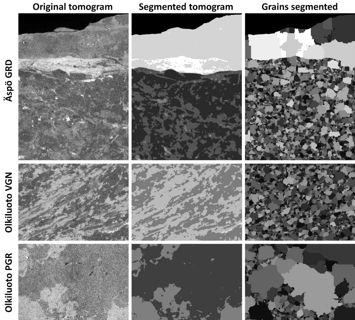
Fig. 6 The cross sections of the original tomographic image (left column), and tomographic images with segmented mineral phases (middle column) and grains (right column). The cross sections for LTDE-SD-GDR1 (upper row), REPRO-VGN (middle row) and REPRO-PGR (lower row) are shown. The mineral phases were segmented based on the gray values in the original image and grains were segmented using the watershed algorithm. The content of different mineral phases and the gray values used in the middle column are given in Table 3. In the right column each segmented grain is given a random gray value.
