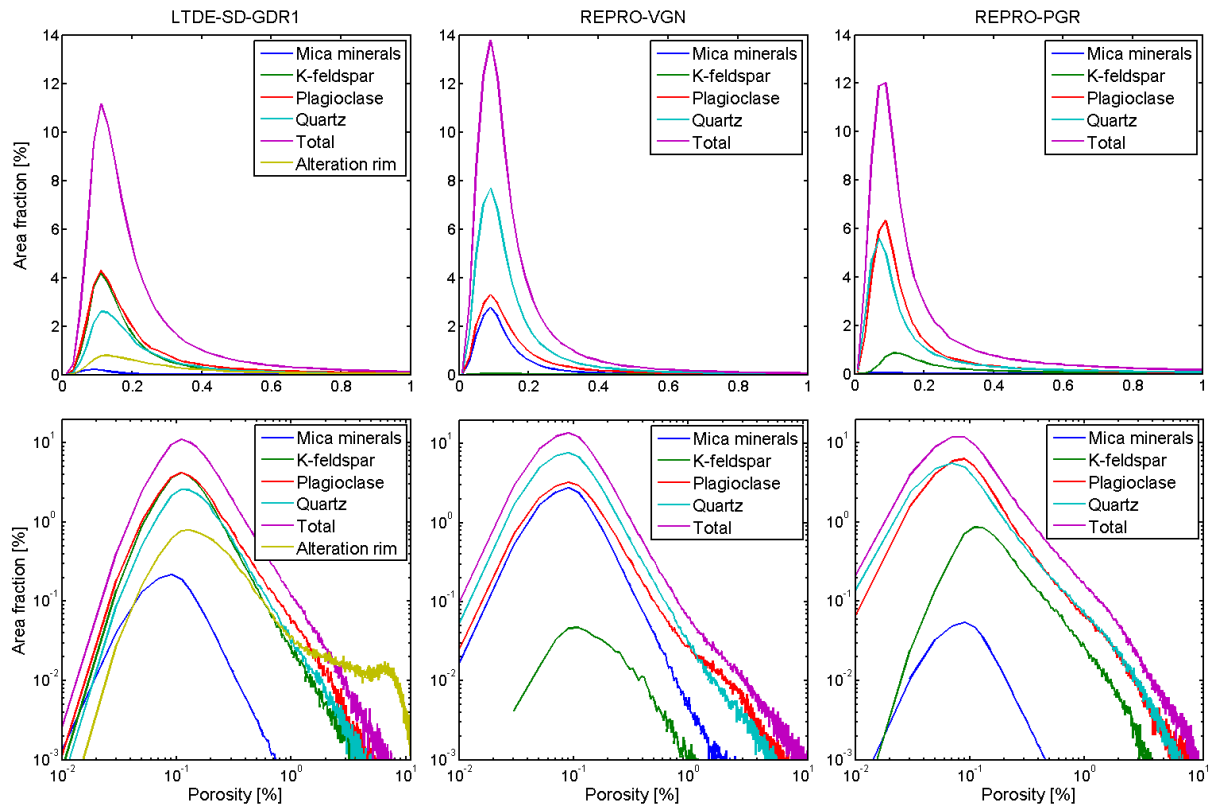
Fig. 5 Porosity histograms of LTDE-SD-GDR1 (left column), REPRO-VGN (middle column), and REPRO-PGR (right column) samples in linear (upper row) and log-log (lower row) scale. The histograms were determined using 20 \mu\text{m} resolution C-14-PMMA autoradiographs (the original and segmented) and a binning of 0.02 %.
