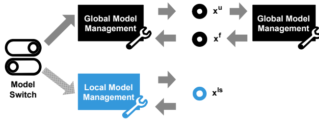
Fig. 12. Model management strategy in CAL-SAPSO.
