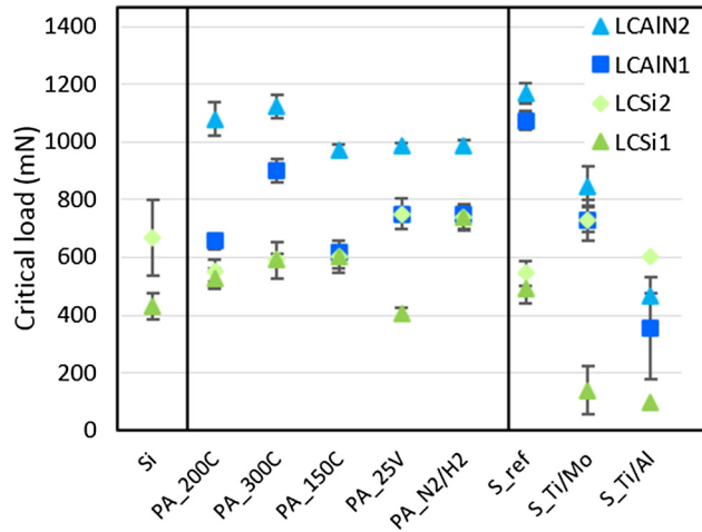
FIG. 4. Critical load values in microscratch testing for the uncoated silicon (Si), ALD films, and sputter deposited films. L_{CSi1} refers to the first observed crack in the Si substrate, L_{CSi2} refers to the beginning of the continuous cracking of the Si substrate, L_{CAIN1} is the first observed local delamination of the coating, and L_{CAIN2} is the continuous delamination of the coating.
