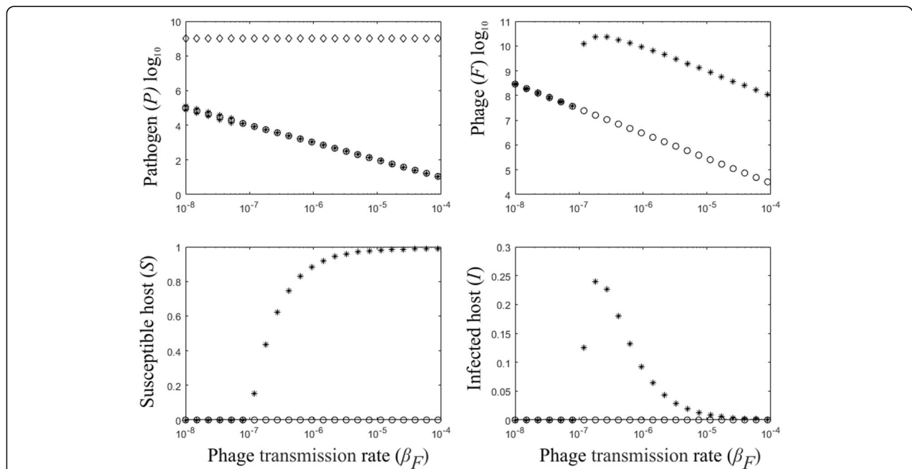
Fig. 1 Bifurcation diagrams of the model dynamics in the absence of the phage-resistant bacteria population ( B = 0 ), presenting equilibrium values of the susceptible host ( S ), the infected hosts ( I ), the pathogen ( P ) and the bacteriophage ( F ) population densities for the phage transmission rate, 10^{-8} < \beta_F < 10^{-4} . The x-axis is log10 scale. When the phage transmission rate is low ( \beta_F < 10^{-7} ), the susceptible and the infected hosts go asymptotically extinct while there is a stable coexistence of the pathogen and the phage. When the phage transmission rate increases, the pathogen population size decreases while the susceptible host population increases, close to their carrying capacity at higher phage transmission rates. The number of the infected hosts abruptly increases as phage transmission increases, but decrease asymptotically towards zero at higher phage transmission rates. The parameter values used are shown in Table 1. Pathogen level in the absence of the host and phage is indicated by “ \diamond ”. The coexistence equilibria of the pathogen and the phage in the absence of the host are denoted by “ o ”. The equilibrium solutions of all populations in the presence of the phage are denoted by “ ** ”
