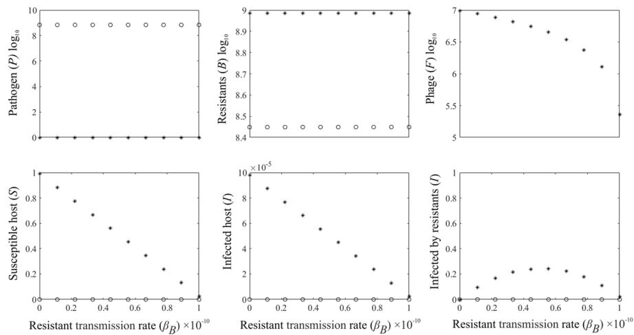
Fig. 3 Bifurcation diagrams of the model dynamics with a competing pathogenic phage-resistant bacteria population. The panels represent the pathogen ( P ), the phage-resistant ( B ) the bacteriophage ( F ), susceptible host ( S ), the non-resistant infected hosts ( I ), the phage-resistant infected hosts ( I_r ), population densities for the phage-resistant transmission rate to the susceptible hosts, 0 < \beta_B < 10^{-10} . The x-axis is log10 scale. When the phage is absent (o) the pathogens drive the host extinct. When the phage is introduced into the system (*) pathogen P is driven on a low level. Now, the abundance of the pathogen B drives the disease dynamics. With increasing infectivity the host population size decreases. The number of the diseases caused by pathogen P remains low due to the phage-control. The disease occurs still due to the increased abundance of the pathogen B . However, the increased infectivity on \beta_B ultimately drives the host population extinct. The parameter values used are shown in Table 1
