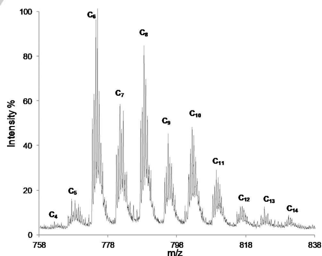
Figure 5. ESI-MS profile for the competition experiment of guests ranging from C_4 to C_{14} (1 eq. of each guest) in the presence of 1 equivalent of cage 1a \cdot Cu . Each isotopic pattern labelled with C_n represents the inclusion complex C_n@1a \cdot Cu
