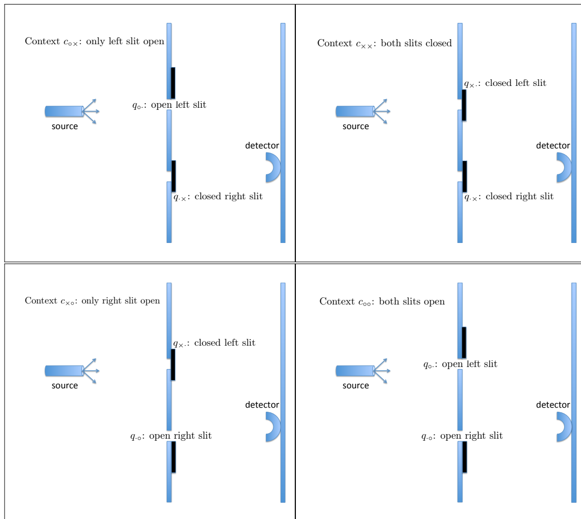
Figure 1. Idealized double slit experiment. The source shoots a single particle that may or may not pass through the slits cut in the intermediate plate, and may or may not be recorded by the detector placed on the screen behind the plate. Each of the slits can be open or closed, and each of the four closed-open arrangements of the two slits forms a context. Each slit (left or right) in each state (open or closed) forms a content, formally treated as the property of the physical system measured by a random variable in a given context.
