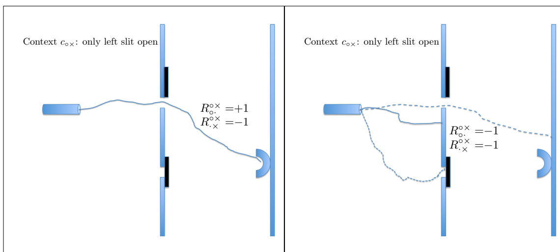
Figure 2. The only physical constraint adopted in our analysis is that a particle can only hit the detector if it has passed through an open slit. The random variables in context c_{o \times} are R_{o,x}^{o,x} (has the particle passed through the open left slit and hit the detector?) and R_{.x}^{o,x} (has the particle passed through the closed right slit and hit the detector?). The physical constraint we impose implies that R_{.x}^{o,x} = -1 with probability 1, which, in turn, implies that in context c_{o \times} the only outcomes that can have nonzero probabilities are as shown in the two panels. The solid irregular curve shows a possible “trajectory” of a single particle, and dashed lines show other possible “trajectories”.
