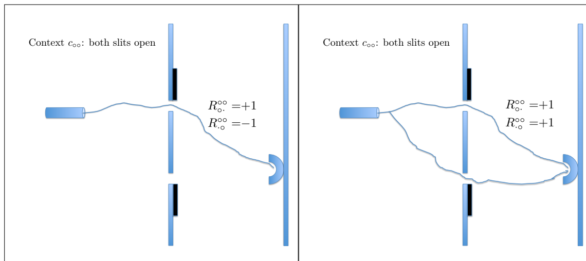
Figure 4. In context c_{oo} , a particle can hit the detector having passed through one of the open slits ( left panel ), but we also allow for the possibility that it passes through both slits ( right panel ), or passes through them several times (not shown). The reason for this is that the outcome of the contextuality analysis does not depend on the probability of the situation in the right panel.
