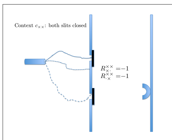
Figure 3. The two random variables in context c_{\times \times} can only attain the values -1 . The situation shown therefore occurs with probability 1.
