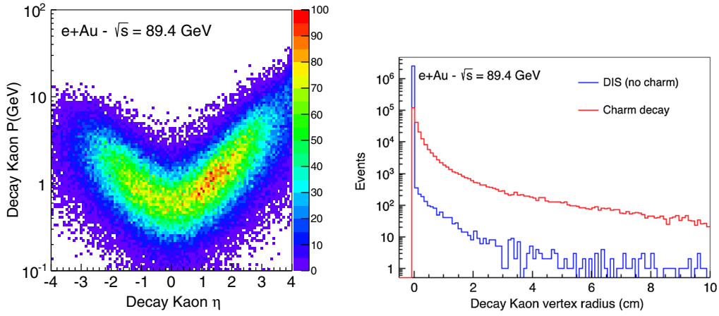
FIG. 5. Left: The distribution of the momentum of a decay K from c\bar{c} production events versus pseudorapidity. Right: The vertex position of K in inclusive DIS (blue line) compared to c\bar{c} production events (red line).
