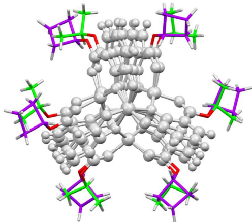
Figure 7. Overlaid structures of the isopropyl \text{Li}[\text{Li}_3(\mathbf{1c})_6\text{Ti}_2] (green) and the cyclo-butyl derivatives \text{Li}[\text{Li}_3(\mathbf{4a})_6\text{Ti}_2] (magenta) showing similar sizes of the ester substituents.
