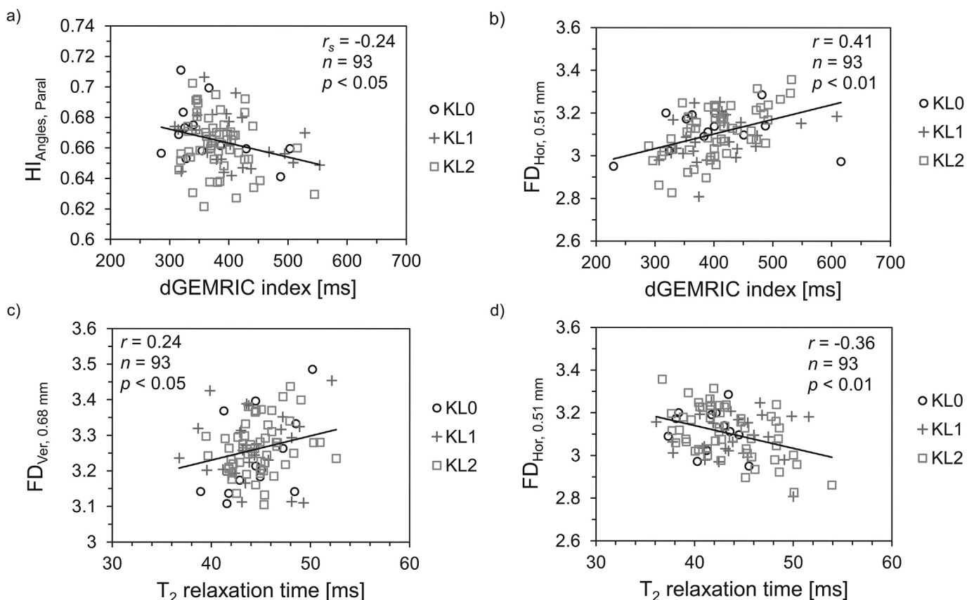
Fig. 2. Statistically significant correlations between (a) HI_{Angles,Paral} in medial subchondral bone and dGEMRIC index of medial tibial cartilage, (b) FD_{Hor,0.51\text{ mm}} in lateral subchondral bone and dGEMRIC index of lateral tibial cartilage, (c) FD_{Ver,0.68\text{ mm}} in medial subchondral bone and T_2 relaxation time of medial tibial cartilage and (d) FD_{Hor,0.51\text{ mm}} in lateral subchondral bone and T_2 relaxation time of lateral tibial cartilage.
