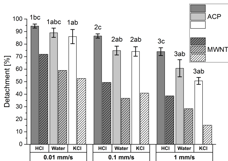
Figure 4: Bar chart summarizing the results of our experiments on detachment of MWNTs and the ACPs in response to interfaces of plain water, 1M KCl solution and 0.01M HCl solution (pH = 2) with three different immersion velocities. The error bars show the standard deviations among the samples. ANOVA-classifications are indicated above the bars for the detachment of ACPs. Numerals refer to the comparison of different immersion velocities for a given immersion solution, while letters point to the comparison of the different solutions for a given velocity. It can be seen that different immersion velocities give systematically rise to statistically significant differences in particle detachment regardless of the immersion solution, while the differences between the solutions are typically not meaningful
