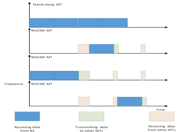
Fig. 2. Transmission process
