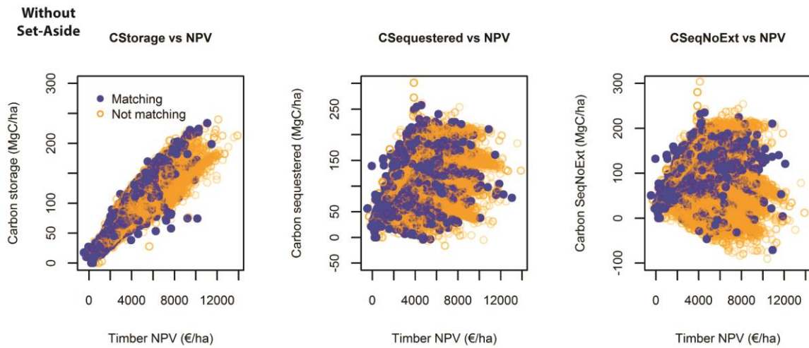
Fig. S3. Scatterplots that indicate the forest stands for which the management regime (excluding set-aside) to maximize timber and each one of the carbon measurements is the same ( matching , blue colour) or is not the same ( not matching , orange).
