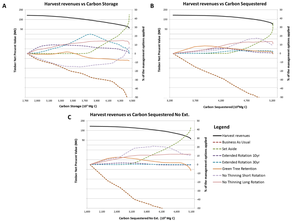
Fig. S5. Changes in the proportion of the seven alternative management regimes with increased levels of carbon in the Pareto optimal sets. Changes are given for each one of the three carbon measurements (A: CStor; B: CSeq; C: CSeqNoExt). Left-hand end of the x-axis refers to cases where harvest revenues (NPV) are maximized (see first row of Table 4 for the reference proportion of management regime at this point). Y-axis describes how much or less each management regime should be applied with increased levels of carbon.
