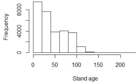
Fig. S1. Histogram showing the distribution of stand age in the study area at the initial conditions.
