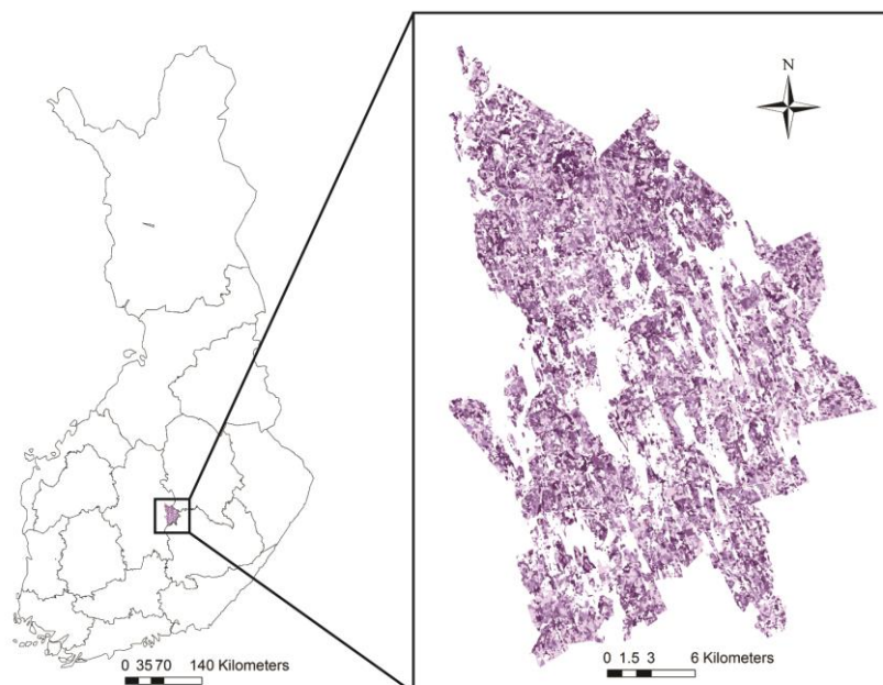
Fig. 1. Map of the location of the study area in Finland.
