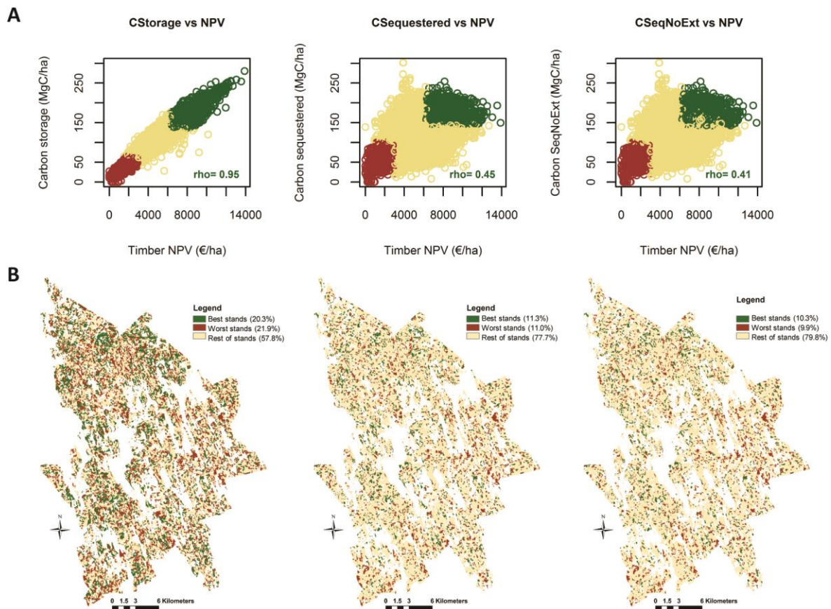
Fig. 2. Scatterplots and spatial patterns for each carbon measurements. The scatterplots (A) indicate the forest stands for which the highest values across all management options for both harvest revenues and each one of the carbon measurements were obtained ( best stands, dark green colour) and the forest stands for which the lowest values for both harvest revenues and each one of the carbon measurements were obtained ( worst stands, dark red colour). Moreover, the Spearman's correlation results ( \rho values) indicate the level of agreement between the harvest revenues and the three different carbon measurements. The maps (B) represent the location of the best , worst and the rest of the forest stands (yellow colour) in the study area.
