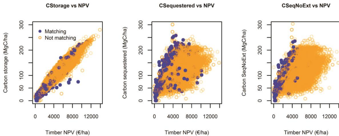
Fig. 4. Scatterplots that indicate the forest stands for which the management regime to maximize timber and each one of the carbon measurements is the same ( matching , blue colour) or is not the same ( not matching , orange colour).
