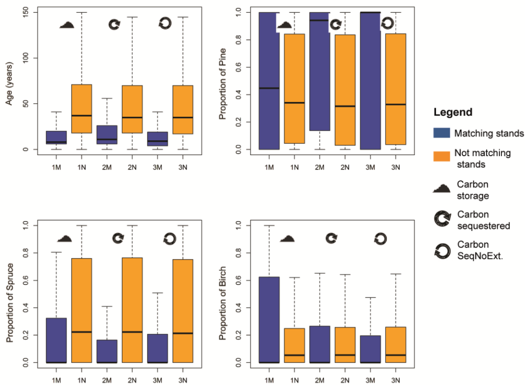
Fig. S4. Boxplots comparing the forest stand characteristics (age and proportion of biomass for the three main tree species) between the matching and the not matching stands for the three carbon measurements (where M refers to matching stands and N to not matching stands; 1 refers to values for NPV and carbon storage; 2 refers to values for NPV and carbon sequestered and 3 refers to values for NPV and carbon sequestered non extracted).
