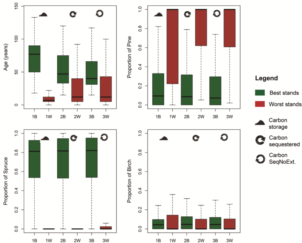
Fig. 3. Boxplots comparing the forest stand characteristics (age and proportion of biomass for the three main tree species) between the best and the worst stands for the three carbon measurements (where B refers to the best stands and W to the worst stands; 1 refers to values for NPV and carbon storage; 2 refers to values for NPV and carbon sequestered and 3 refers to values for NPV and carbon sequestered non extracted).
