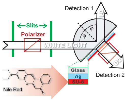
FIG. 1. (Color online) Schematics of the measurement setup and the samples. The sample is mounted on the flat surface of the rotatable hemicylindrical prism by index matching oil. The excitation of SPPs is done by linearly polarized and collimated white light and both the reflected signal (detection 1) and the luminescence signals (detection 2) were collected to a fiber guiding the radiation to a spectrometer. \varphi is the angle of incidence as well as the detection angle in detection 1. The lower left part represents the structure of the sample consisting of two layers, silver and SU-8 polymer with the Nile Red dye embedded, at the top of a glass substrate. Thickness of the silver and polymer layers were about 50 nm.
