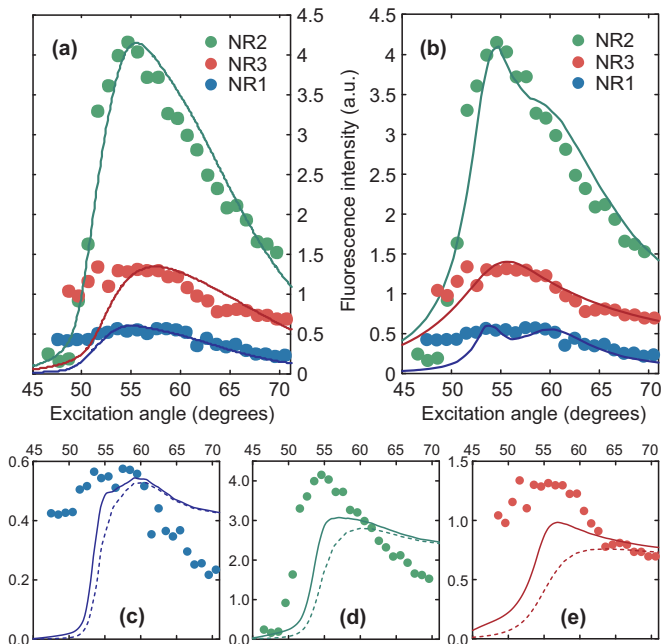
FIG. 5. (Color online) Fluorescence as a function of the incoming angle. (a) Measured total fluorescence (circles) for the three samples NR1 (blue), NR2 (green), and NR3 (red), together with the theoretical transfer matrix calculations (solid lines). (b) Measured total fluorescence (circles) together with the results of the quantum mechanical three-state model (solid lines). (c)–(e) Measured total fluorescence (circles) of (c) NR1, (d) NR2, and (e) NR3 together with the results of the three-state model including relaxation and thermalization of the polariton modes (dashed lines), as well as decoherence via thermalization (solid lines).
