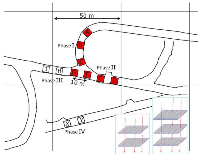
Figure 2. Layout of EMMA in the mine caverns 75 metres below ground. Phase I – IV refer to the four branches of the array and the detector stations are indicated by red rectangles (those of white have not been installed yet). The central stations C, F and G have three detector layers, each 1125 mm apart, while the rest have two, as illustrated in two insets bottom right.
