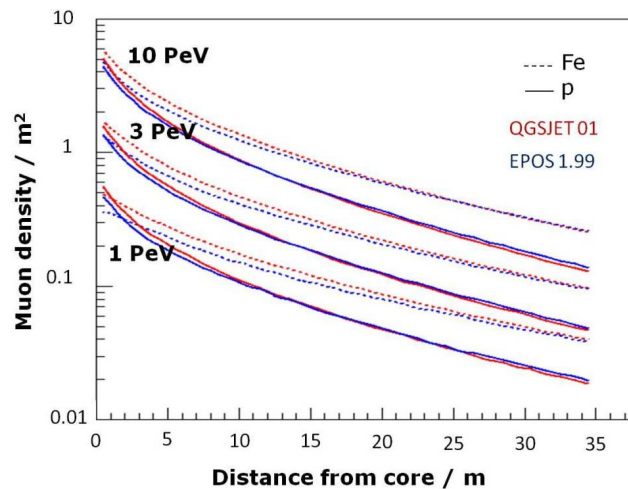
Figure 1. Simulated lateral muon density distributions of high-energy muons ( E_\mu > 50 GeV) of proton and iron-initiated air showers at 1, 3 and 10 PeV energies. CORSIKA+QGSJET 01 and CORSIKA+EPOS 1.99 models indicated by red and blue lines, respectively.
