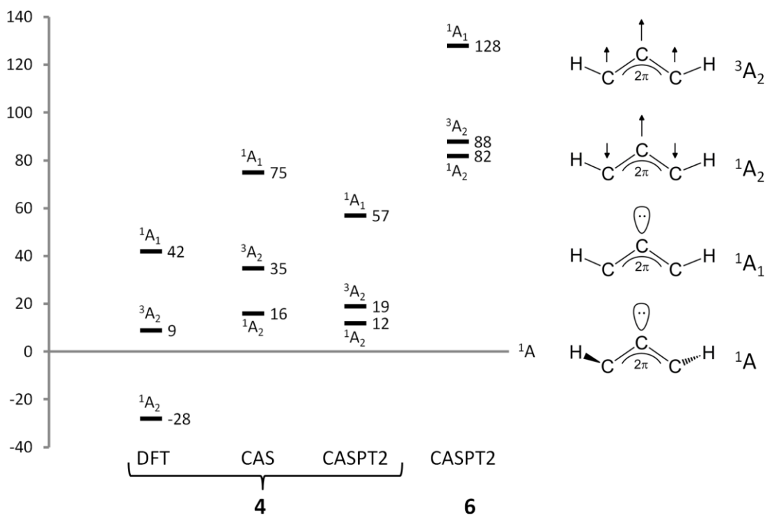
Figure 2. Relative energies (in \text{kJ mol}^{-1} and with respect to the ^1\text{A} state) of the lowest electronic states of 4 and 6 calculated at different levels of theory. Data for compound 6 taken from Reference 28.
