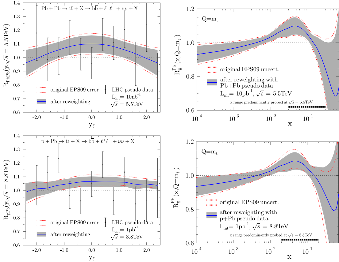
Fig. 4. Impact on the nuclear glue of t\bar{t} (pseudo)data for the full LHC heavy-ion programme. Left: Nuclear modification factor for t\bar{t} decay-leptons as a function of rapidity, R_{\text{ppPb}}(y, \sqrt{s}) , obtained for Pb-Pb at \sqrt{s_{\text{NN}}} = 5.5 TeV (top) and p-Pb at \sqrt{s_{\text{NN}}} = 8.8 TeV (bottom) compared to predictions computed with EPS09: current nPDF set (region enclosed by the red dotted lines) and after pseudodata-reweighting (blue curve plus grey band). Right: Ratio of nuclear-over-proton gluon densities, R_g^{\text{Pb}} evaluated at Q = m_t , for the original EPS09 (band enclosed by red dotted lines) and for the reweighted EPS09 (blue curve with grey band) for Pb-Pb (top) and p-Pb (bottom). (For interpretation of the references to colour in this figure legend, the reader is referred to the web version of this article.)
