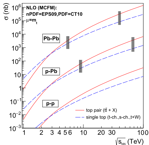
Fig. 1. Total cross sections for top pair and single-top (sum of t -, s -channels plus tW processes) production in Pb–Pb, p–Pb and p–p collisions as a function of c.m. energy. The dashed boxes indicate the nominal nucleon–nucleon c.m. energies, \sqrt{s_{NN}} = 5.5, 8.8, 39, 63 TeV, of the heavy-ion runs at the LHC and FCC.
