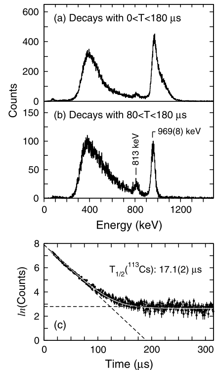
Fig. 1. Panels (a) and (b) show energy spectra from the DSSD. Panel (a) gives the spectrum of decays recorded within 180 \mu\text{s} of an implant. The large peak at \sim 1 \text{ MeV} is attributed to ^{113}\text{Cs} proton decays; the high-energy tail on the peak is due to pile-up of fast decays with the tail of the implant signal. Panel (b) shows decays recorded between 80 and 180 \mu\text{s} after an implant; the pile-up tail is no longer present, allowing the position of the proton-decay peak to be determined to be 969(8) keV. Also apparent on panels (a) and (b) is the peak at 813 keV due to proton decays of ^{109}\text{I} ( T_{1/2} \simeq 100 \mu\text{s} ) and ^{112}\text{Cs} ( T_{1/2} \simeq 500 \mu\text{s} ). Panel (c) gives the time between implant and decay in the DSSD, gated on the 969-keV peak; the data give a half-life of 17.1(2) \mu\text{s} .
