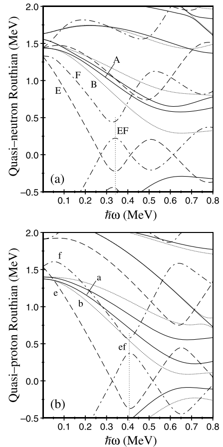
Fig. 4. Quasiparticle Routhians from Woods-Saxon cranked-shell model calculations for (a) neutrons and (b) protons. The calculations are performed for a deformation of \beta_2 = 0.20 , \beta_4 = 0.04 , and \gamma = 0^{\circ} . The different line styles represent values of parity and signature, (\pi, \alpha) , as follows: dashed lines (1, -1/2); dot-dashed lines (-, +1/2); solid lines (+, +1/2); and dotted lines (+, -1/2). The two lowest negative- and positive-parity quasiparticles, are labelled using the standard nomenclature. The positions of the lowest alignments for neutrons [EF; panel (a)] and protons [ef; panel (b)] are marked by faint vertical dotted lines.
