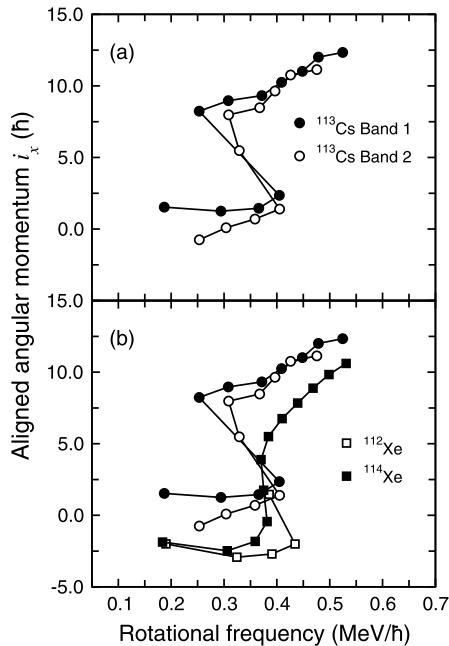
Fig. 5. Aligned angular momenta of the two rotational bands in ^{113}\text{Cs} , shown in comparison to neighboring even–even Xe isotopes. For all data points a reference configuration with Harris parameters [36] of \mathcal{J}_0 = 17.0 \text{ MeV}^{-1}\hbar^2 and \mathcal{J}_1 = 25.8 \text{ MeV}^{-3}\hbar^4 has been subtracted. Panel (a) shows data for both bands in ^{113}\text{Cs} . Panel (b) shows the ^{113}\text{Cs} data in comparison to the ground-state bands of ^{112,114}\text{Xe} . The legend on panel (a) also applies to panel (b). The data for ^{112,114}\text{Xe} are taken from Refs. [37,38] and the data for ^{113}\text{Cs} are from the present work.
