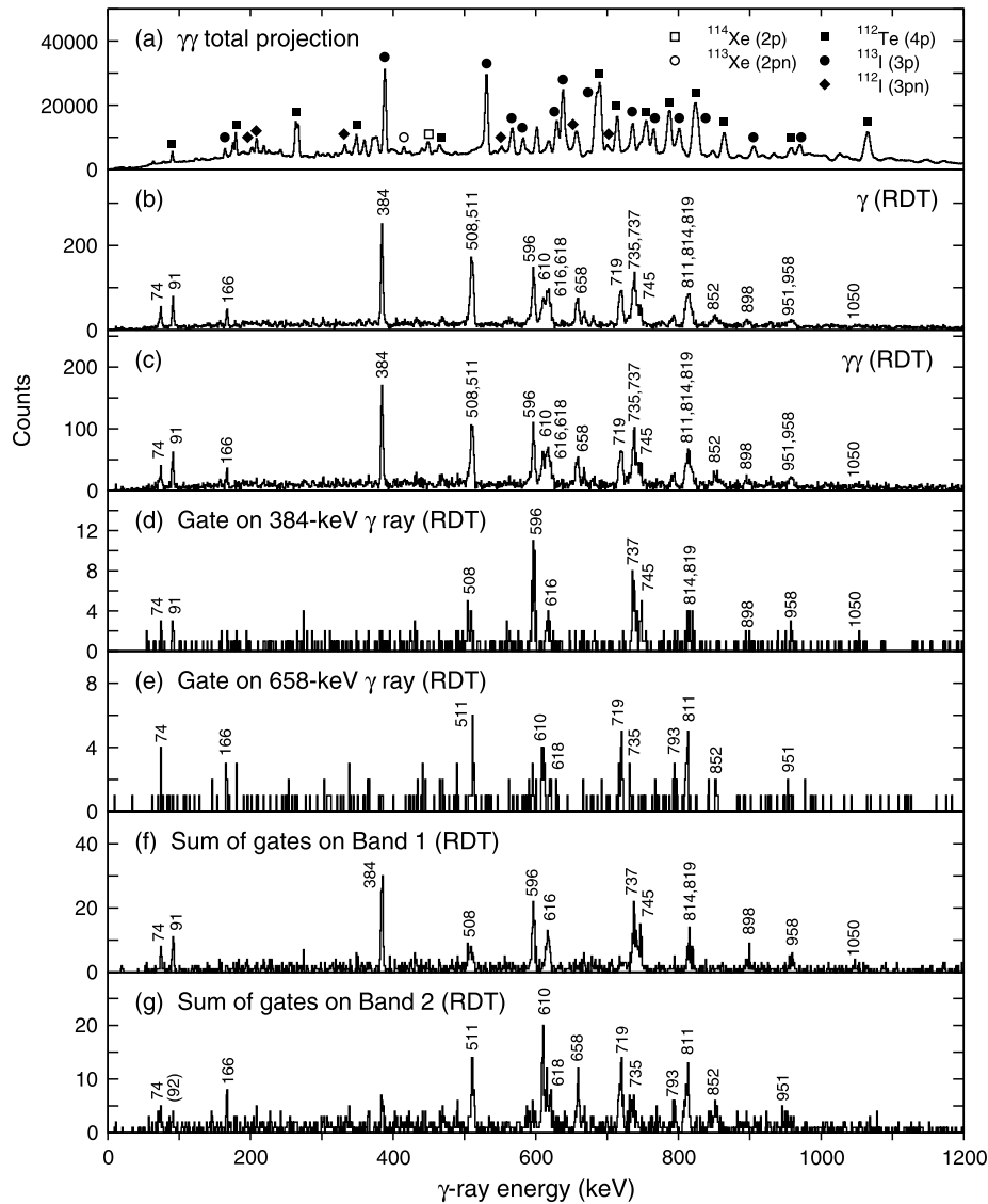
Fig. 2. Gamma-ray spectra recorded in this work. Panel (a) gives the projection of a \gamma\gamma matrix, incremented by all \gamma rays that are detected in coincidence with an evaporation residue at the focal plane of RITU; the largest peaks in the spectrum correspond to transitions in ^{112}\text{Te} ( 4p evaporation), ^{113}\text{I} ( 3p ), and ^{112}\text{I} ( 3pn ). Panels (b) to (g) show \gamma rays that are tagged with a 969-keV proton being emitted within 100 \mu\text{s} of an implant (RDT gated), in which all of the labelled peaks represent transitions that have been assigned to ^{113}\text{Cs} . Panels (b) and (c) show the \gamma (singles) and \gamma\gamma (doubles) projections, respectively. Panels (d) and (e) show \gamma rays in coincidence with the 384- and 658-keV \gamma rays, respectively, revealing different subsets of the ^{113}\text{Cs} \gamma rays. Panel (f) shows \gamma rays in coincidence with the transitions at 384, 508, 596, 616, or 737 keV; the resulting transitions are assigned to Band 1. Panel (g) shows \gamma rays in coincidence with the transitions at 511, 658, 719, 811, or 735 keV; the resulting transitions are assigned to Band 2. The presence of the (92)-keV transition in panel (g) is discussed in the text.
