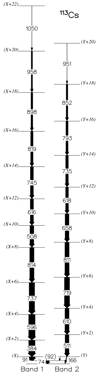
Fig. 3. The level scheme of ^{113}\text{Cs} deduced in the present work. The widths of the arrows are proportional to the relative \gamma -ray intensities. The values in parentheses are spins relative to the lowest state in each band which have been assigned here as X and Y for Bands 1 and 2, respectively. The spin and parity assignments are discussed in the text.
