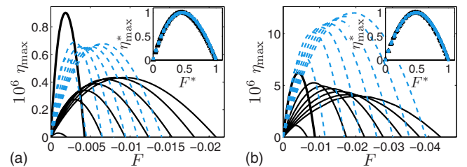
FIG. 5. (Color online) Maximum efficiency for RD (black solid) and FM (blue dashed) polymers as a function of the load force F with N=2\dots 9 in type 1 (left) and type 2 (right) traveling potentials. In each case, the rightmost curve is for N=9 and the bold lines (the less interesting special case N=2 ) are shared for both RD and FM polymers. (Insets) Rescaled data \eta_{\max}^* as a function of F^* , with black triangles for RD polymers and blue squares for FM polymers.
